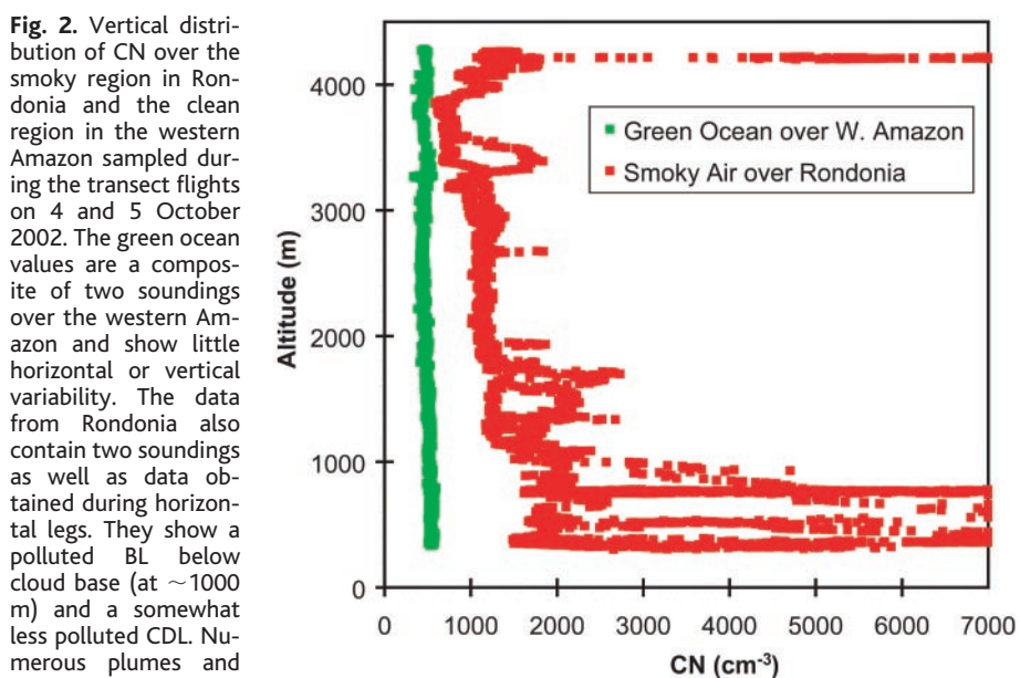
Fig. 2. Vertical distribution of CN over the smoky region in Rondonia and the clean region in the western Amazon sampled during the transect flights on 4 and 5 October 2002. The green ocean values are a composite of two soundings over the western Amazon and show little horizontal or vertical variability. The data from Rondonia also contain two soundings as well as data obtained during horizontal legs. They show a polluted BL below cloud base (at \sim 1000 m) and a somewhat less polluted CDL. Numerous plumes and haze layers are embedded in both the BL and the CDL. The layer at 4.2-km altitude had a minimal horizontal extent of about 12 km.
