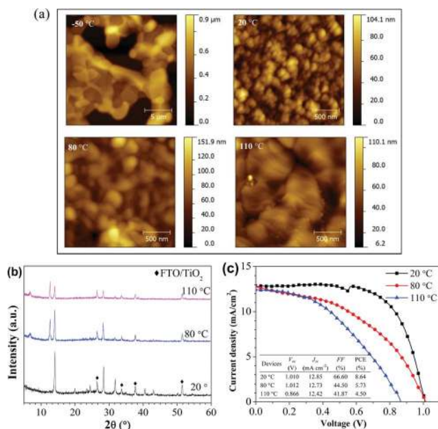
Fig. 6 (a) AFM topography images of perovskite films grown on Si substrates at different substrate temperatures during the hybrid deposition from \text{PbI}_2 : \text{MAI} . The RMS roughness values are 209.9, 9.9, 20.1 and 13.1 nm for -50 , 20, 80 and 110 °C of substrate temperatures, respectively. (b) XRD spectra of perovskite films grown on \text{TiO}_2/\text{FTO} substrates at different substrate temperatures. (c) J - V curves of the devices under 1 sun illumination employing perovskite films prepared at different substrate temperatures. The device structure is \text{FTO}/\text{TiO}_2 (70 nm)/perovskite (110 nm)/spiro-MeOTAD (100 nm)/Au (100 nm). The table as the inset shows the photovoltaic parameters of the devices.
