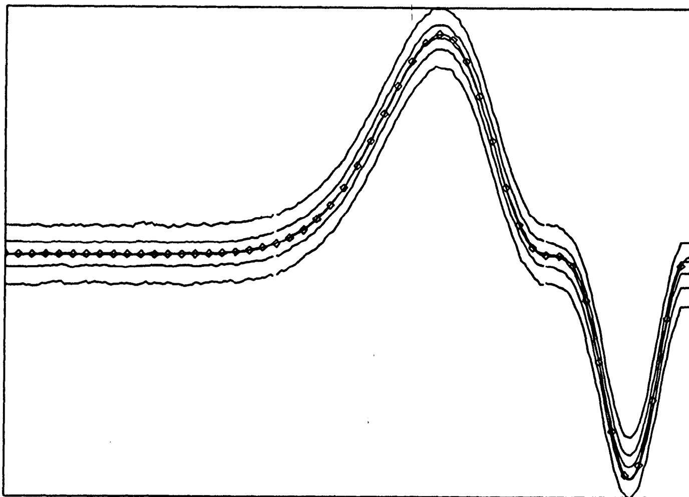
Figure 11: Ensemble of Median Smooths of \sin^3(2\pi x^3)
