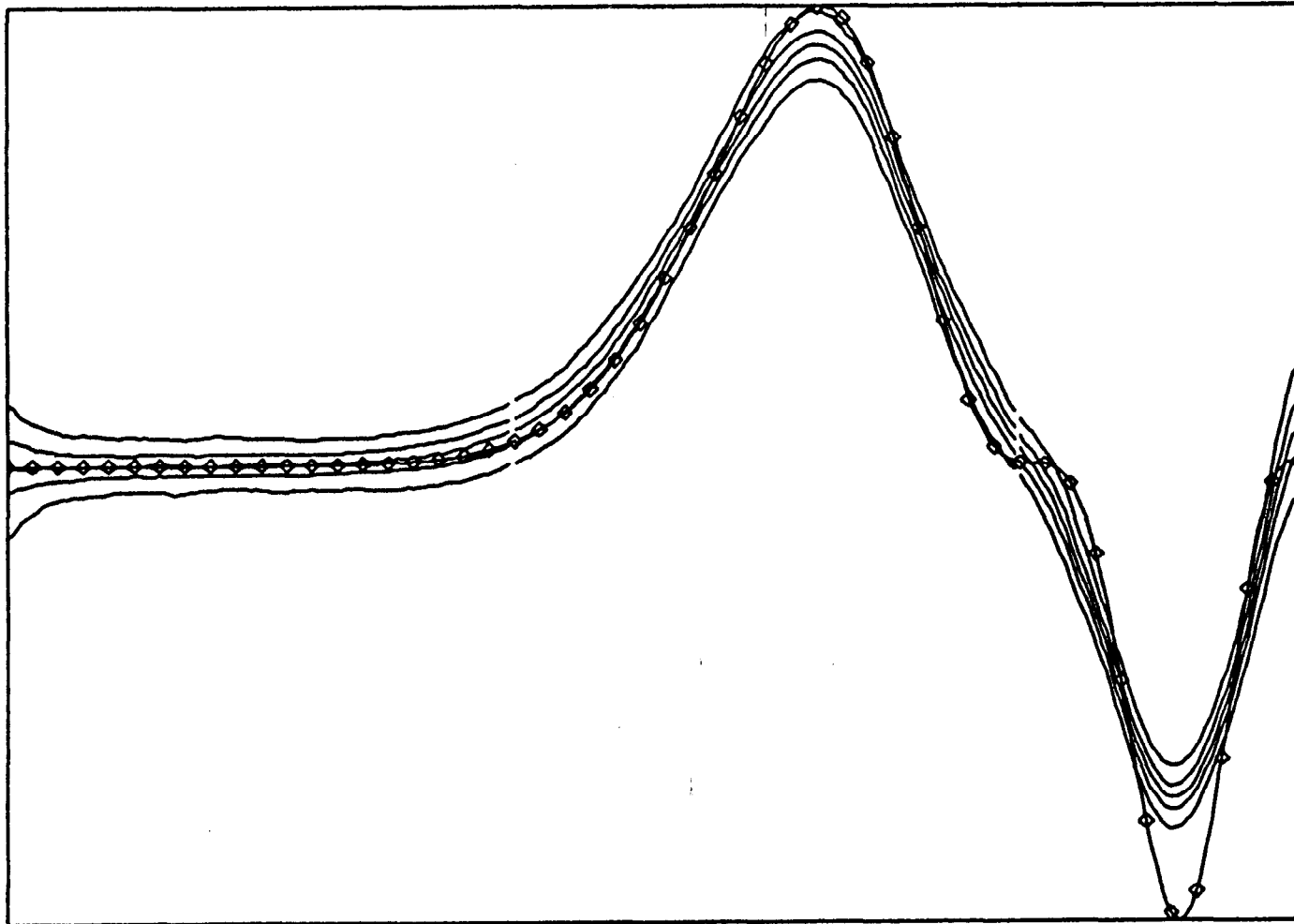
Figure 10: Ensemble of Central Smooths about \sin^3(2\pi x^3)
