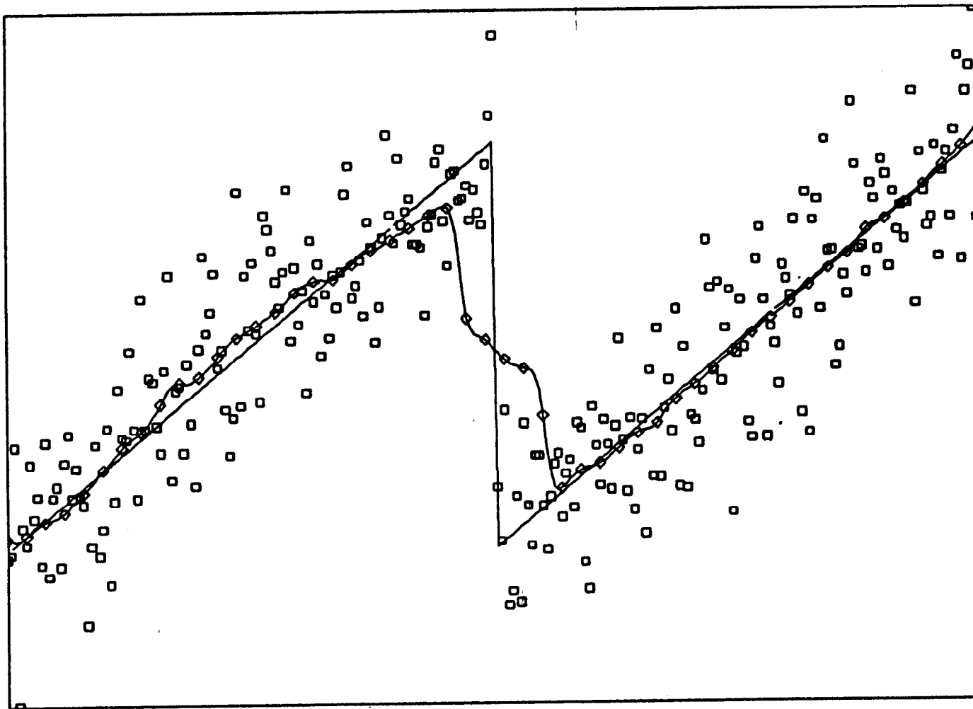
Figure 1: A Central Smooth of a Sawtooth Function with Noise
