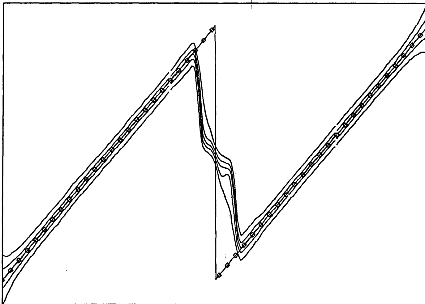
Figure 4: Ensemble of Central Smooths about the Sawtooth Function
