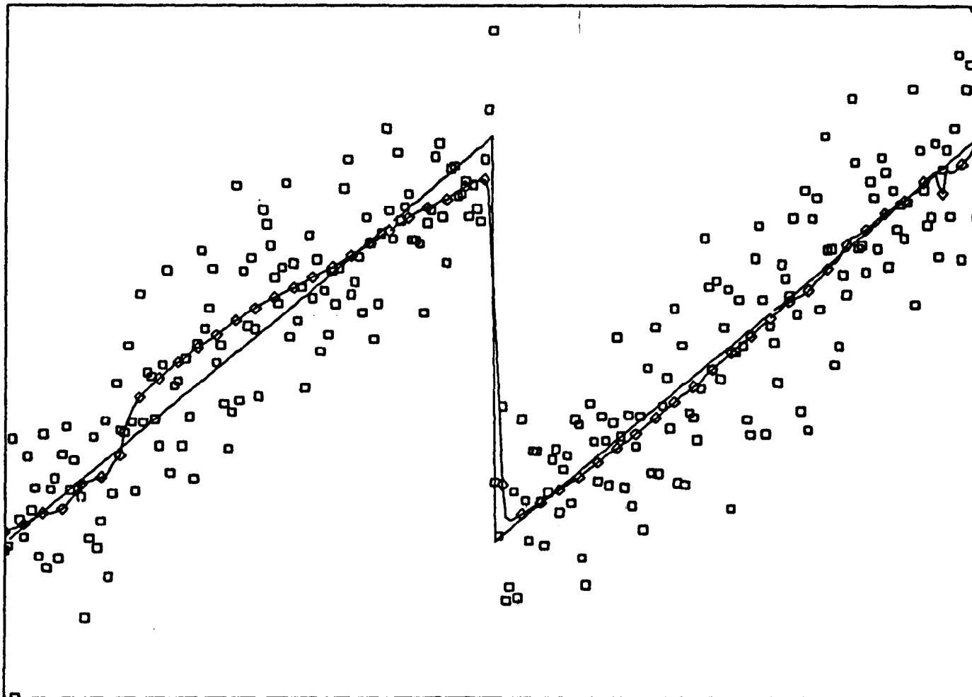
Figure 3: A Split Linear Smooth of a Sawtooth Function with Noise
