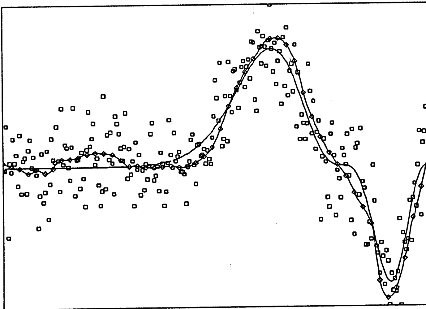
Figure 9: A Split Linear Smooth of \sin^3(2\pi x^3) with Noise
