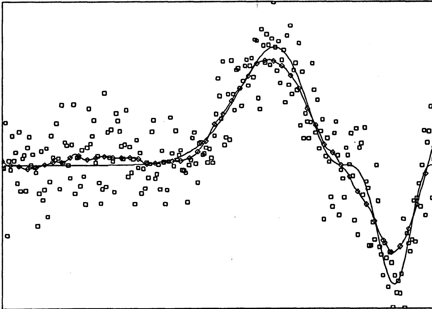
Figure 7: A Central Smooth of \sin^3(2\pi x^3) with Noise
