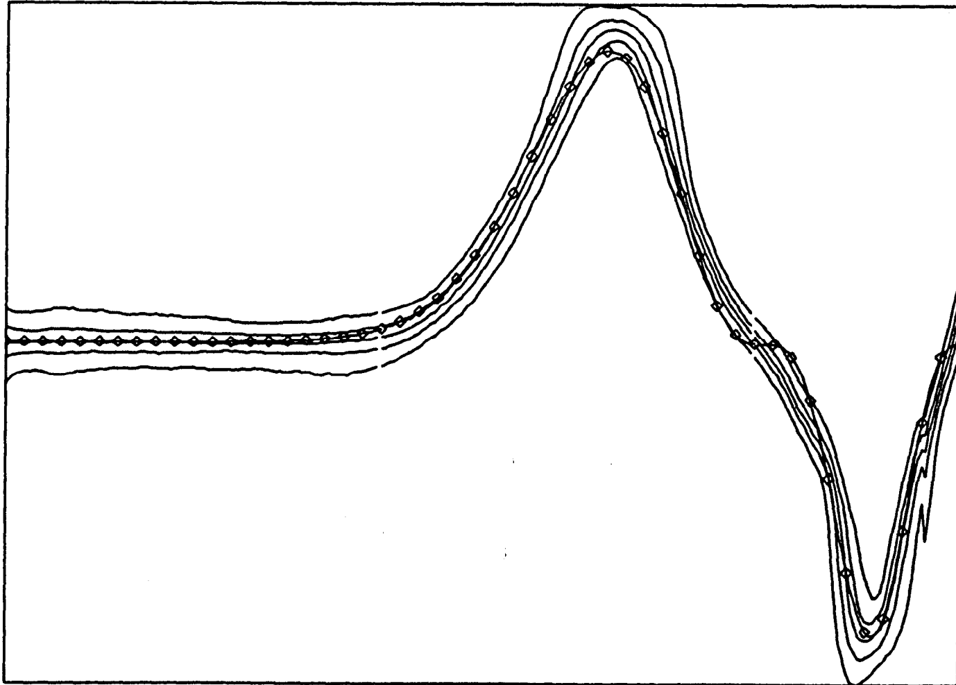
Figure 12: Ensemble of Split Linear Smooths of \sin^3(2\pi x^3)
