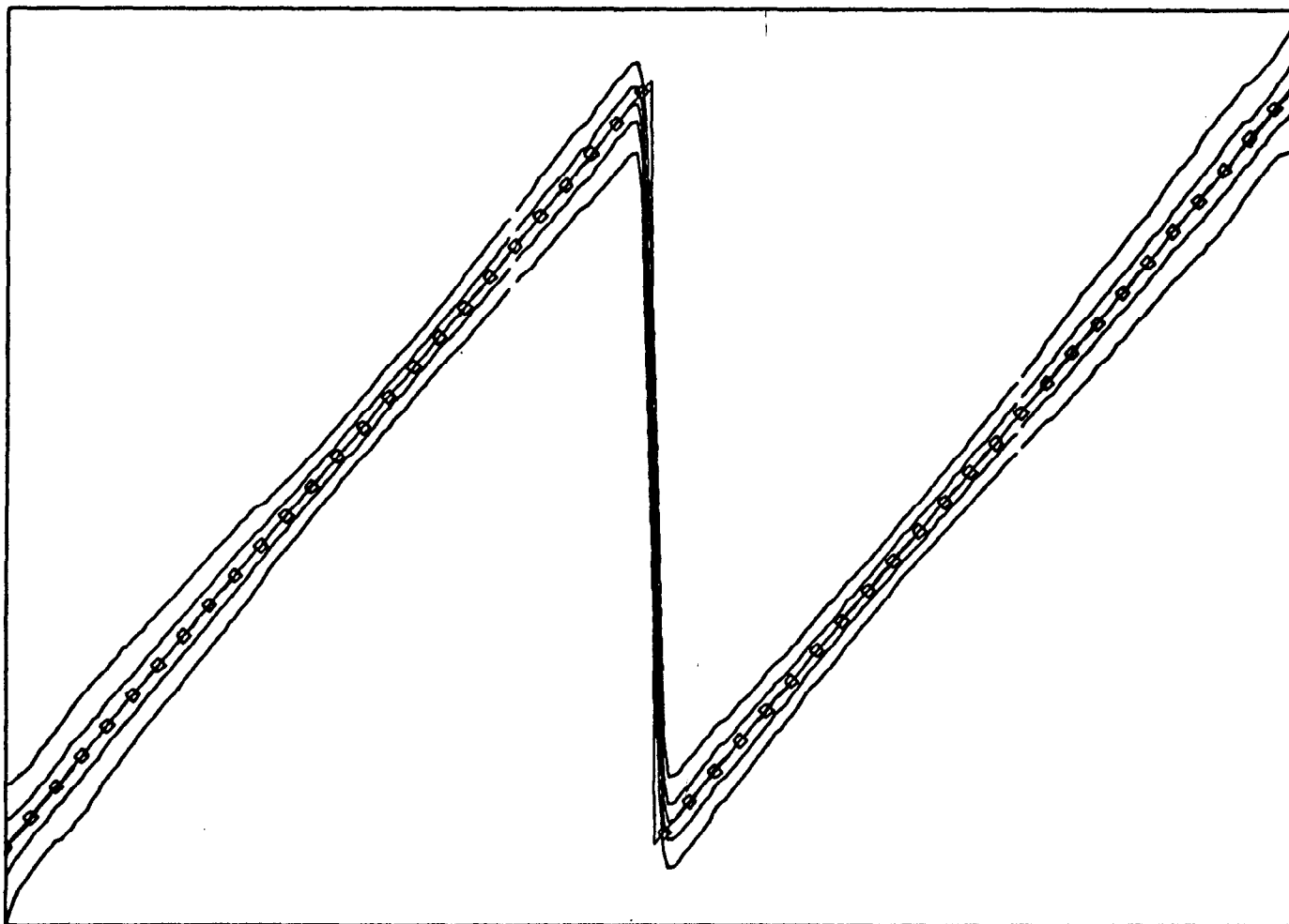
Figure 6: Ensemble of Split Linear Smooths about the Sawtooth Function
