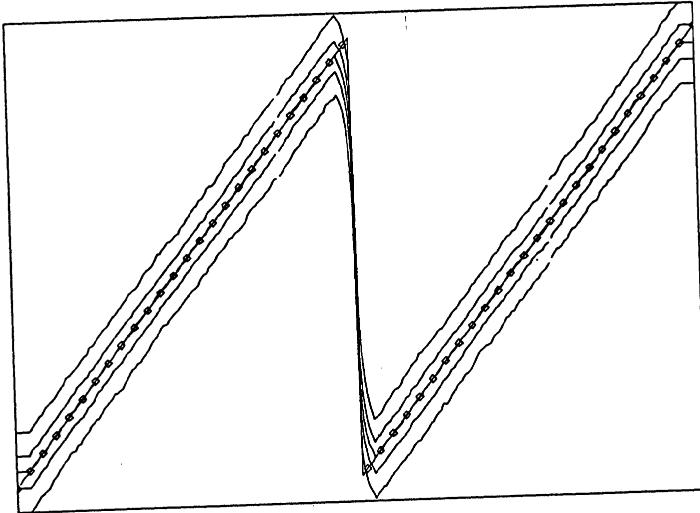
Figure 5: Ensemble of Median Smooths about the Sawtooth Function
