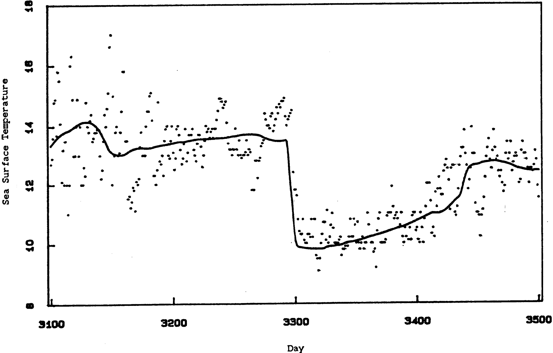
Figure 14: Close-up of Spring Transition in Sea Surface Temperature Data
