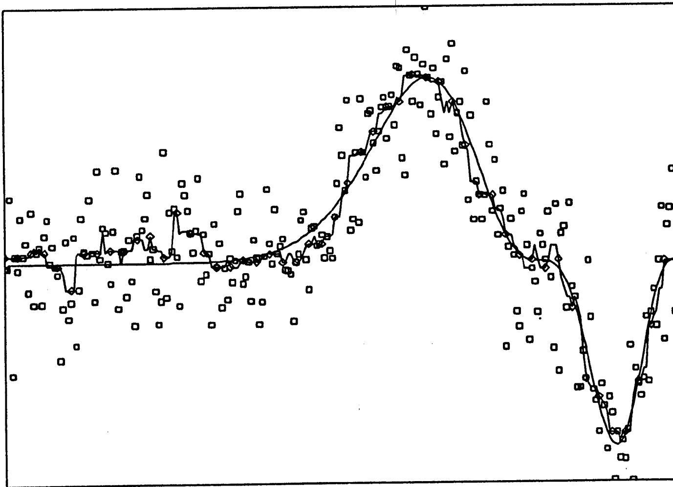
Figure 8: A Median Smooth of \sin^3(2\pi x^3) with Noise
