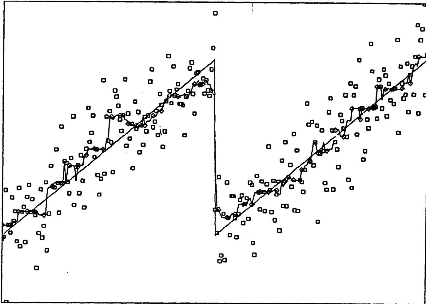
Figure 2: A Median Smooth of a Sawtooth Function with Noise
