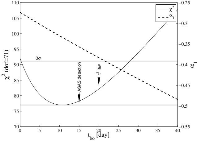
FIG. 10.— \chi^2 (solid line) of the fit of L_{0,\text{obs}}([t-t_{\text{bo}}]/t_{\text{bo}})^\alpha as a function of t_{\text{bo}} . The gray horizontal lines show the minimum \chi^2 and the 3\sigma confidence level assuming three free parameters. The dashed line shows the value of \alpha_1 (the power-law index of the optical slope in the first year) as a function of t_{\text{bo}} , where its values are presented in the right-hand ordinate axis.
