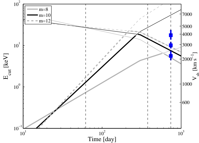
FIG. 13.— The predicted X-ray cutoff energy (Eq. 26) as a function of time. Different line types and gray-scale levels are for different values of m as indicated in the legend. The heavy lines represent the minimum function (Eq. 26), while the thin lines represent the two possibilities in Equation 26 without taking the minimum. The blue squares show the temperature as measured in the NuSTAR+XMM epoch (Table 6; faint sources removed). The upper square is for the zvpshabs*mekal model, the bottom square refers to zvpshabs*powerlaw*spexpcut , and the square in the middle is for zvpshabs*powerlaw*spexpcut with \Gamma = 1 . The vertical dashed lines show the epochs of the two Chandra and the NuSTAR+XMM observations. The right-hand ordinate axis gives the shock velocity corresponding to the cutoff energy, based on Equation 25.
