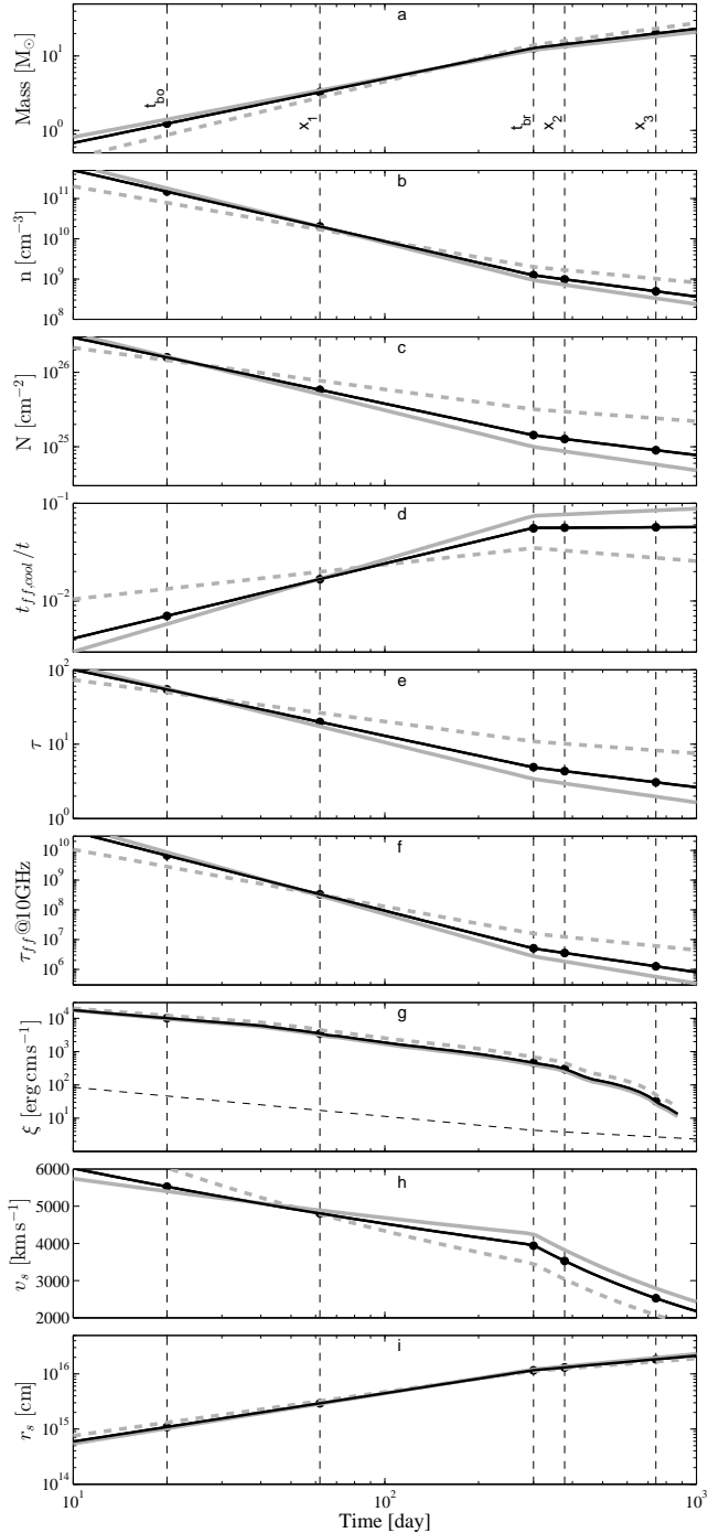
FIG. 12.— The CSM properties as a function of time, assuming t_{bo} = 20 day and m = 10 (black lines). The gray lines are for m = 12 , while the dashed-gray line is for m = 8 . The black-dashed vertical lines show the breakout time scale ( t_{bo} ), the time of the optical light-curve break (300 days; t_{br} ), the times of the first two Chandra epochs ( x_1 and x_2 ), and the XMM+NuSTAR epoch ( x_3 ). The different panels show the following: (a) CSM mass within the shock radius and the observer, (b) density of the CSM at the shock radius, (c) column density between the shock and the observer, (d) free-free cooling time scale divided by the time at the shock radius, (e) Thomson optical depth between the shock radius and the observer, (f) 10 GHz free-free optical depth, (g) ionization parameter (Eq. 28), (h) shock velocity, and (i) shock-radius evolution. Time is measured relative to maximum I -band light minus t_{bo} . We note that panel (g) shows an additional dashed black line; it represents the minimal ionization parameter (for m = 10 ) as estimated by replacing the luminosity in Equation 28 by the observed X-ray luminosity ( L_X \approx 1.5 \times 10^{41} erg s ^{-1} ). The intrinsic X-ray luminosity may be much higher because of, for example, bound-free absorption.
