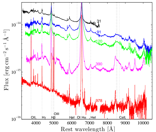
FIG. 2.— Selected visible-light spectra of SN 2010jl. The number near each spectrum marks its age in days (see Table 2). The last spectrum taken on day 978 may be contaminated by emission from the underlying star-forming region.
