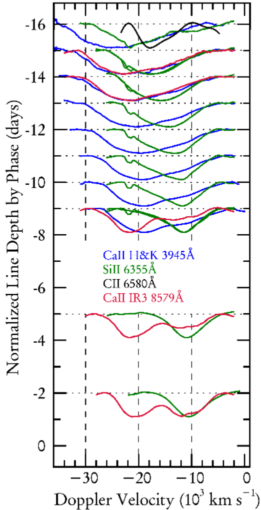
FIG. 8.— The evolution of absorption features C II (black), Si II (green) and Ca II (blue and red) in pre-maximum spectra of SN 2012cg. The features are normalized to a flat continuum and the line depths are normalized to 1.0. These line profiles identify the locations of line forming regions for each ion in velocity space. C II is only measurable at -16 d. Si II exhibits a detached HVF at -16 d and strong influence of the HVF in Si II line profiles at -14 d and -13 d. HVF of Ca II are common in SN Ia, and here they persist until at least -2 d.
