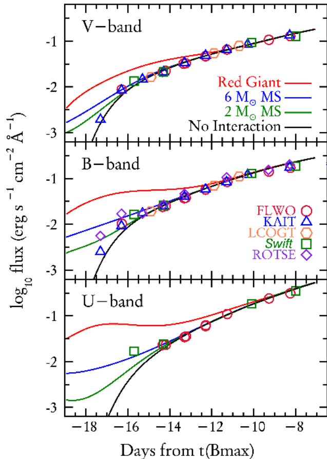
FIG. 6.— Early U -, B - and V -band data for SN 2012cg are plotted with model results for a normal SN Ia with no interaction and 3 cases of interaction with a binary companion (Kasen 2010). The models fit the data well at phases after -14 d (except for the Red Giant model (red line) that is divergent through about -11 d). When the model light curves separate, the model for a SN Ia with no interaction (black) has the lowest predicted flux. Data obtained before -14 d are brighter than predicted by the normal models and the closest model fit is for interaction with a 6 M_{\odot} MS star (blue line). The values of the earliest KAIT points (blue triangles) are somewhat uncertain (see §4 for more information).
