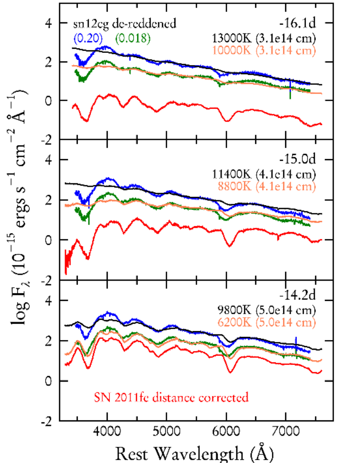
FIG. 9.— The earliest spectra of SN 2012cg are dereddened and plotted in blue for Host + MW extinction and green for MW only. The spectra plotted in red are distance corrected SN 2011fe spectra from similar phases. The black and orange spectra are the SN 2011fe data with blackbodies added at the temperatures and radii listed in each panel. Dilution of the features consistent with adding continuum to the spectra of SN 2011fe. Note that the BB radii are approximately the same as the photospheric radii at these phases. The SN 2012cg spectra are bluer and hotter than spectra of SN 2011fe at comparable phases which is consistent with the photometric measurements. At -14.2d , the red spectrum is offset by -0.2 \text{ log flux units} to make it easier to see the orange and green spectra.
