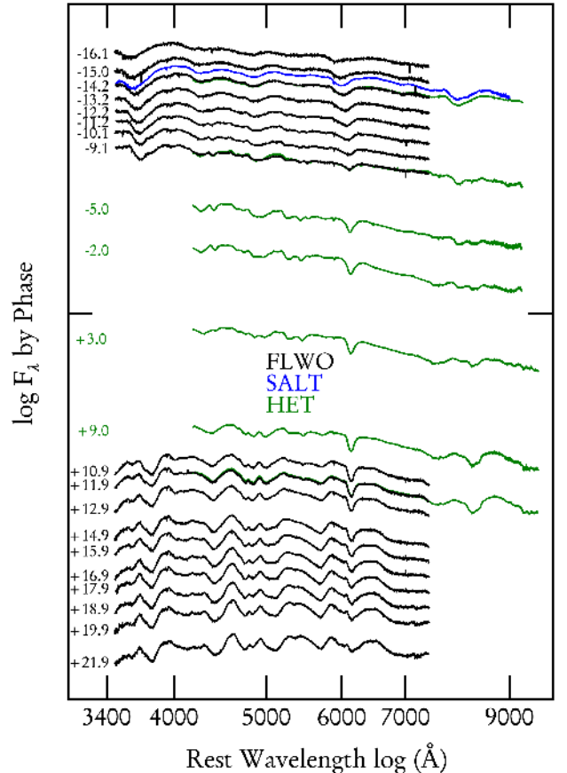
FIG. 3.— Optical spectroscopy of SN 2012cg obtained from -16.1 d to +21.9 d. The sources are FLWO (black), SALT (blue) and HET (green). The continuum slopes of the spectra show that SN 2012cg is a blue SN Ia at early phases. Absorption features in the pre-maximum spectra are relatively weak. This is characteristic of slightly overluminous SN Ia.
