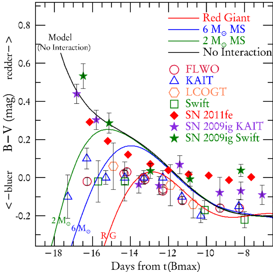
FIG. 7.— B - V colors for the SN 2012cg are displayed using open symbols. The colored lines trace B - V for the interaction models. B - V data for two normal SN Ia are plotted using filled symbols: SNe 2009ig (Foley 2013, stars) and 2011fe (Pereira et al. 2013, diamonds). The colors for the other two SN are similar to the model for a normal SN Ia with no interaction (solid black line) but they do not fit the data for SN 2012cg or any of the interaction models. The colors for SN 2012cg are much bluer at the earliest phases, they redden for 2 – 3 days and then “turn over” near -15 d. After reaching this peak, the SN 2012cg colors follow the normal track. The B - V data for SN 2012cg are closest to the model with a 6 M_{\odot} companion (blue line).
