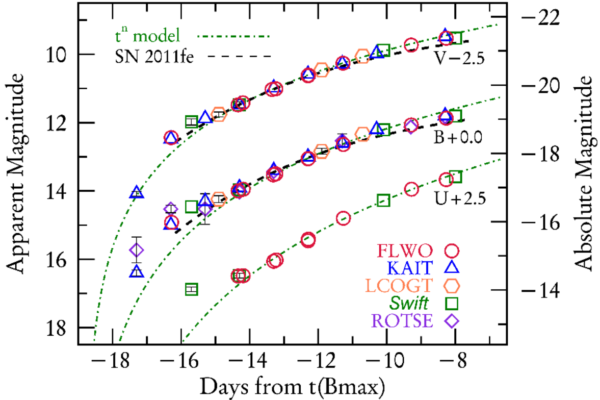
FIG. 4.— V -, B - and U -band photometry (top to bottom) of SN 2012cg from multiple sources. The data have been corrected for extinction. The LC of SN 2011fe (Vinko et al. 2012, dashed black lines) stretched to yield a rise time of 18.8 days equivalent to SN 2012cg (see text) and t^n model LCs (dot-dash, green) are plotted as templates for a normal SN Ia. The power-law indices used for different bands are 3.4 ( U ), 2.4 ( B ) and 2.2 ( V ), see text for details. In all bands, the SN 2012cg data display excess flux at phases earlier than -14 d. From -14 d toward maximum light, the data from SN 2012cg and SN 2011fe fit the templates well. Uncertainties are marked only where they approach the size of the symbols. Note that uncertainties on the earliest KAIT points are likely underestimated (see §4 for more information).
