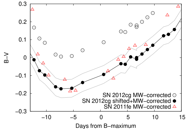
FIG. 2.— B - V color evolution for SN 2012cg and SN 2011fe after correction for Milky Way (Galactic) reddening. The curves are fit to minimize the difference near t(B_{max}) . We assume that SN 2011fe has essentially zero reddening, so the magnitude of the difference determines E(B - V)_{host} \approx 0.18 mag. (See Section 2.)
