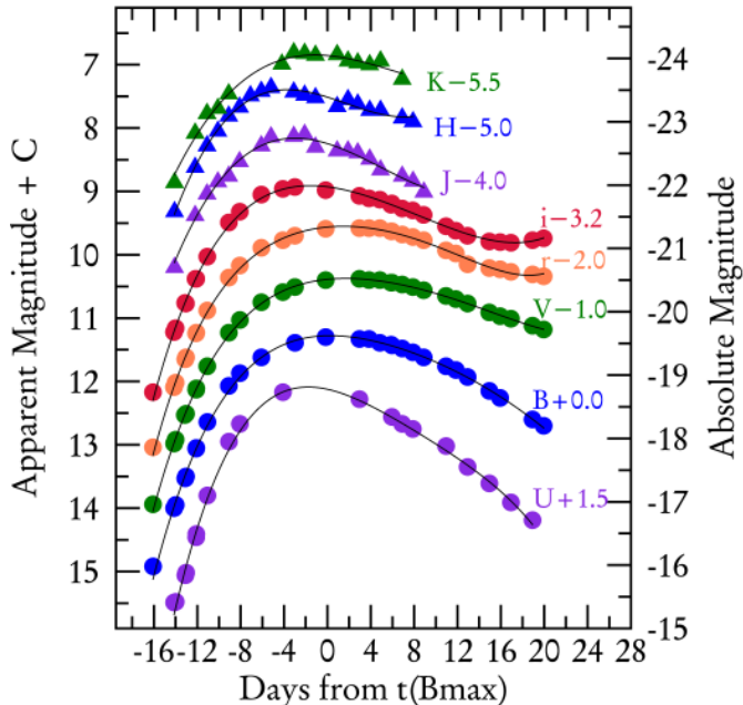
FIG. 1.— UBVr'i'JHK_s photometry of SN 2012cg obtained at the F. L. Whipple Observatory from -16.1 d to +19.9 d. The data are corrected for MW and host galaxy extinction. The black lines are polynomial fits used to identify the peak brightness and the time of peak for each filter (Table 1). We find t(B_{max}) = 560681.3 (MJD) = June 3.3 (UT), with a peak magnitude in the B -band of -19.62 mag and \Delta m_{15}(B) = 0.86 .
