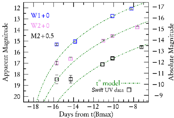
FIG. 5.— Swift photometry (squares) for SN 2012cg obtained in UV filters: W1 , M2 and W2 . The data have been corrected for extinction. Excess flux is apparent at -16 d in all filters, and it is also present at -14 d for M2 and W2 . Model LCs scaled as t^{3.6} (see text) are plotted for reference in each passband with green dot-dashed lines. The timing of the observed UV excess matches well with the optical data displayed in Figure 4.
