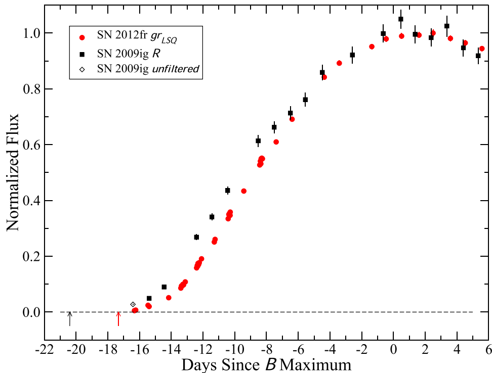
Figure 19. Relative fluxes (normalized to maximum) plotted as a function of the time with respect to t_{B,max} for the R -band light curve of SN 2009ig and the gr_{LSQ} light curve of SN 2012fr. The photometry for SN 2009ig is taken from (Foley et al. 2012). The unfiltered first observation was approximately S-corrected assuming a color (B - V) = 0.6 \pm 0.1 and a sensitivity function similar to those of the Tarot and BOSS unfiltered photometry. The black arrow shows the last non-detection before discovery for SN 2009ig and the red arrow shows the same for SN 2012fr. The abscissa is corrected for time dilation.
