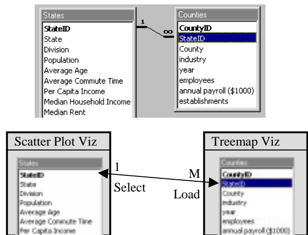
Figure 2: Top: A schema diagram for a database of Census information for U.S. states and counties (using Microsoft Access).
