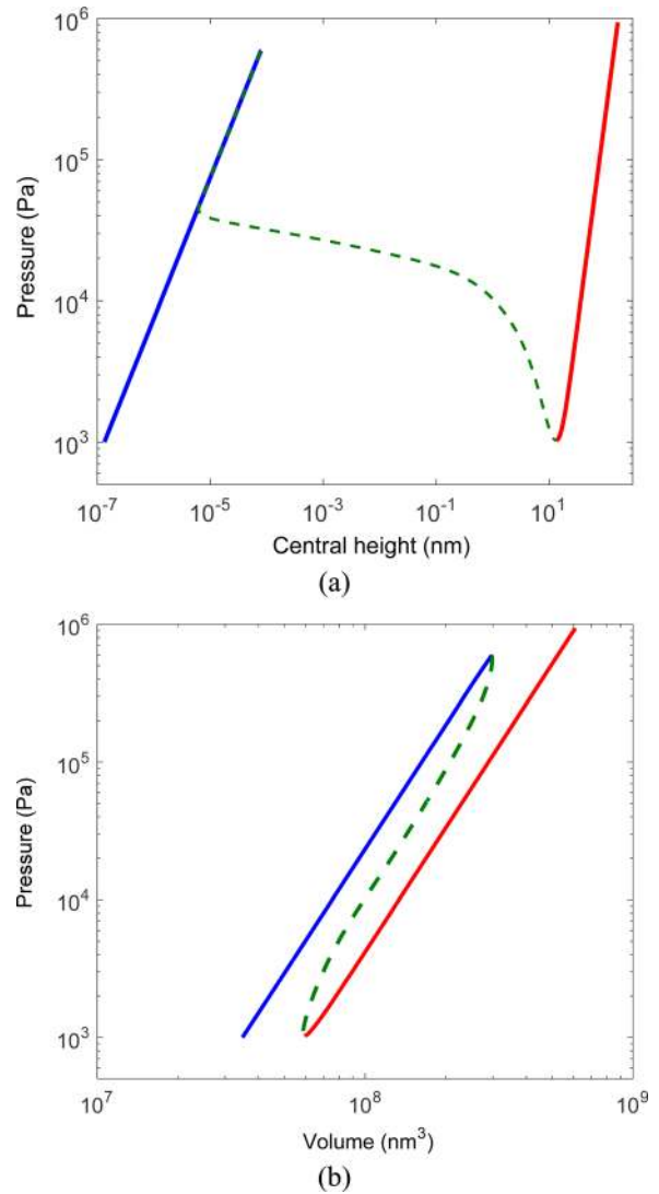
Fig. 8 (a) Central height versus pressure and (b) volume versus pressure for a center-island graphene blister ( a = 1.5 \mu\text{m} and b = 0.25 \mu\text{m} )
