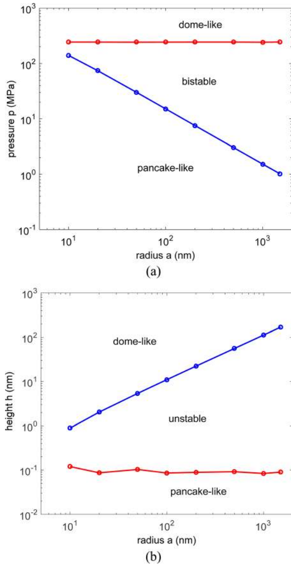
Fig. 7 Phase diagrams for graphene bubble blisters: (a) pressure versus radius and (b) height versus radius
