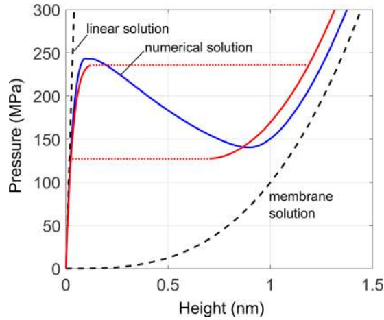
Fig. 17 Comparison of the approximate two-state solution by energy minimization with the numerical solution for the pressure–height curve of a graphene bubble blister ( a = 10 \text{ nm} )
