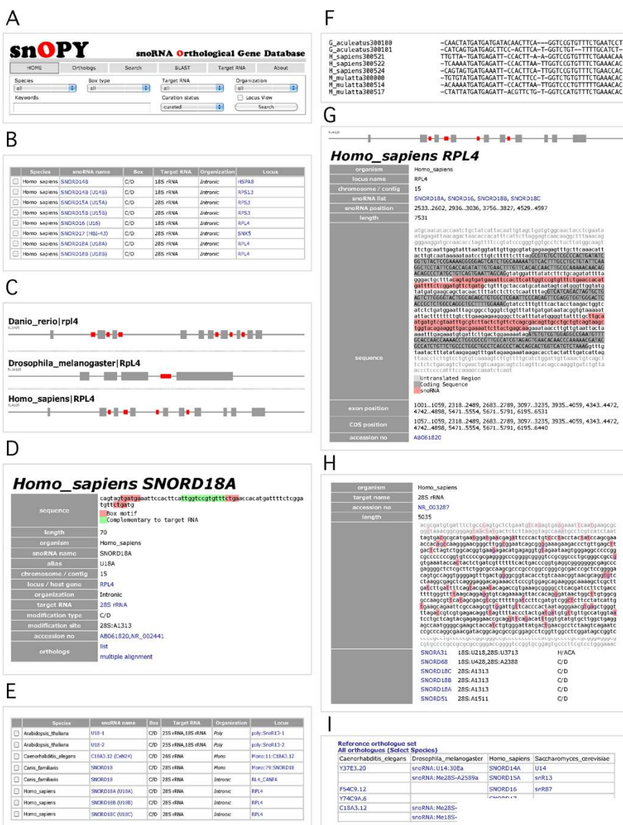
Figure 3 Representative snapshots of snOPY pages. A , search form; B , search results selected with “Homo sapiens”; C , results retrieved from “Locus View” using “RPL4” as a keyword; D , individual snoRNA entry page for H. sapiens SNORD18A, with box motifs and complementary sequences highlighted in red and green, respectively; E , orthologues retrieved using “list” in the human SNORD18A page; F , multiple sequence alignment for SNORD18A; G , snoRNA gene locus of the human RPL4 gene for SNORD18A; H , target RNA and modification sites for human 28S rRNA; I , an orthologue table for four representative species. With the exception of A and C , only a part of each page is shown in the snapshot.
