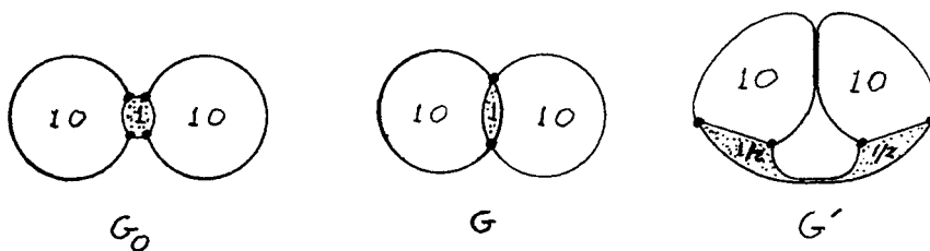
FIGURE 3.2. Given an embedded graph G_0 and prescribed areas A_1 = 10 , A_2 = 1 , A_3 = 10 , Theorem 3.2 provides a least-perimeter deformation G of G_0 . In this figure, two edges of G_0 have degenerated to points in the limit G . In the limit, edges are allowed to bump up against each other, as in the poorer admissible competitor G' . Where two edges coincide, the length counts twice.
