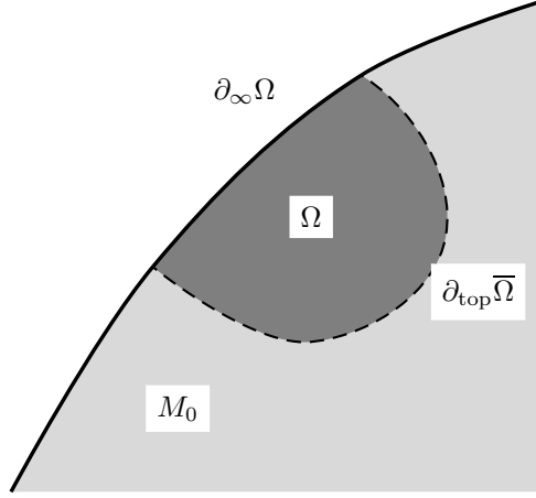
FIGURE 1. A regular open set \Omega . Note that the interior of \partial_\infty\bar{\Omega} is contained in \Omega , but the true boundary \partial_{\text{top}}\Omega = \partial_{\text{top}}\bar{\Omega} is not contained in \Omega
