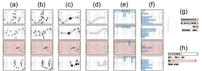
Fig. 11. Available small multiple views: (a) dots, (b) lines and dots, (c) flow and groups, (d) line, (e, f) x and y distribution histograms, (g) alignment by distance travelled, (h) alignment by duration.
