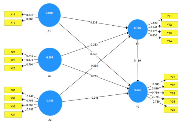
Figure 2. Inner model
