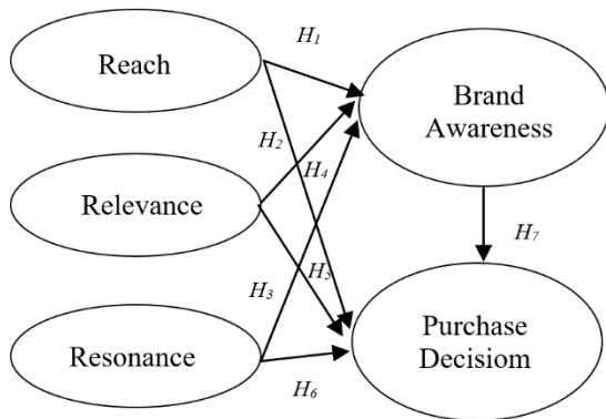
Figure 1. Research model
