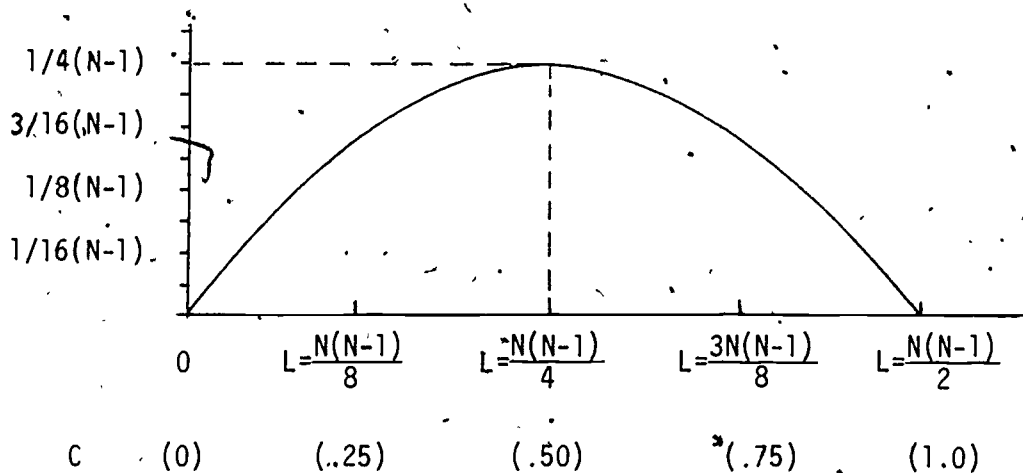
Figure 1b. Generalized plot of expected variance against N and C^S/n (system connectiveness with respect to nodes). Note that the maximum value for S_e^2 of 1/4(N-1) is at the point where C=.50 . At this point, the observed number of links will be one-half of the maximum possible. Note also that all networks, regardless of size ( N ) and linkage ( C ), are described by this single graph. Thus, absolute comparisons between networks are possible with this form of description.
