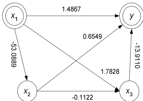
Fig. 5 Network of direct and indirect effects for resources
