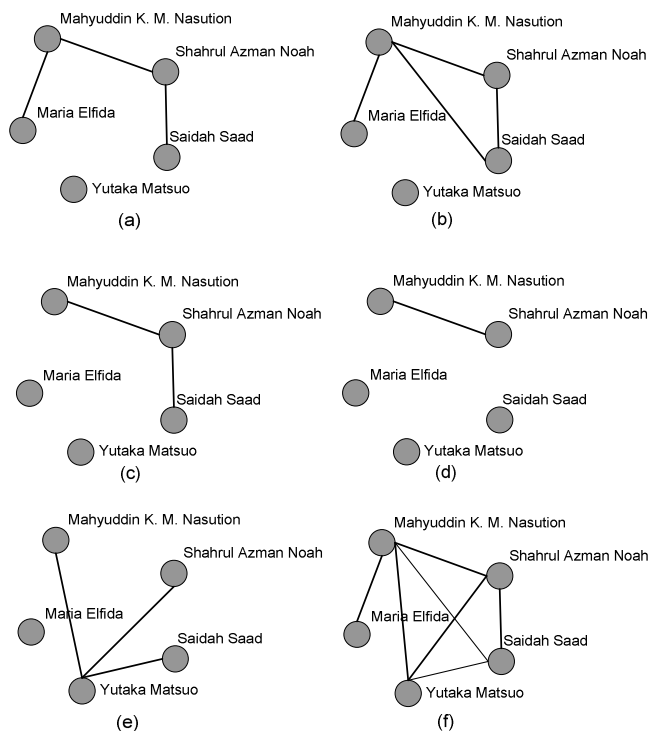
Fig. 1. Some of the relationships among five social actors
