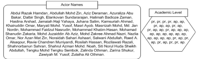
Fig. 3 List of seeds as a sample
