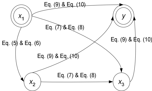
Fig. 4 Network of direct and indirect effects for four factors (resources)
