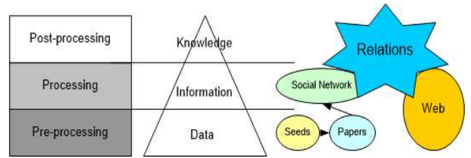
Fig. 2 An approach to defining the relation resources and SNA
