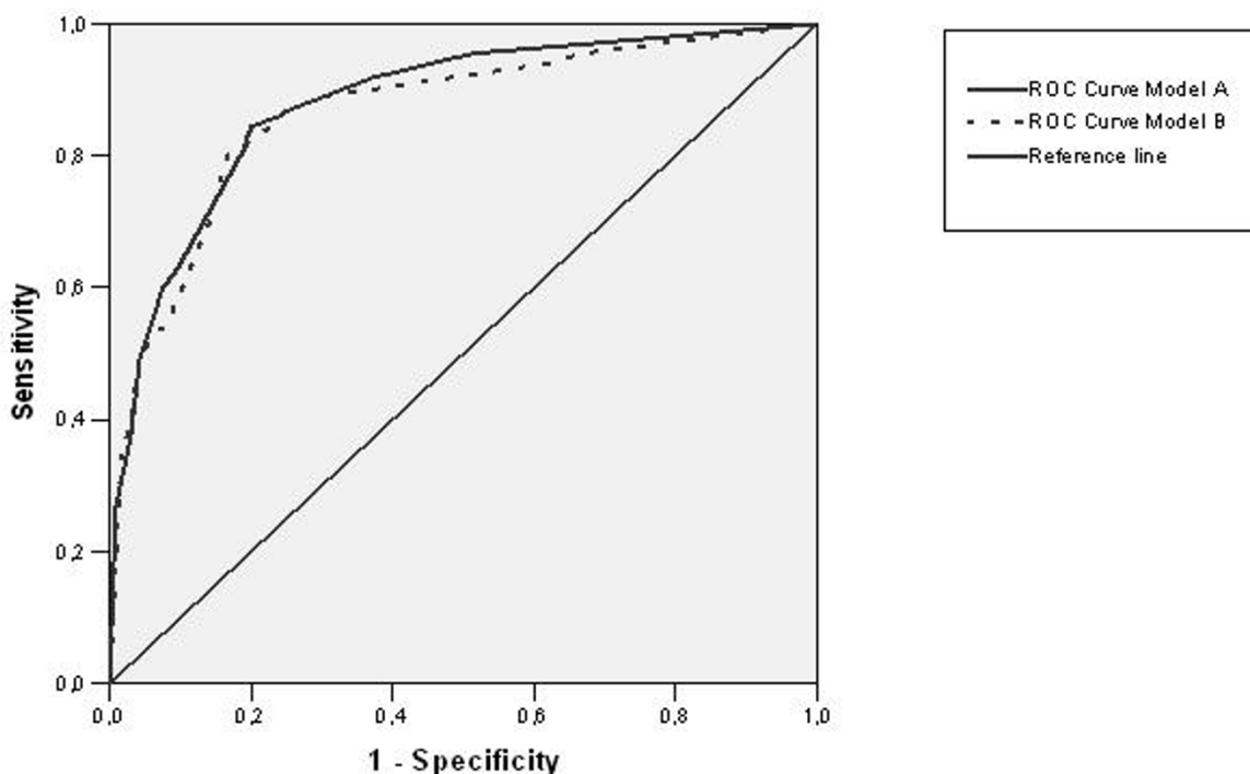
Figure 1 ROC for ADL independence in models A and B.
