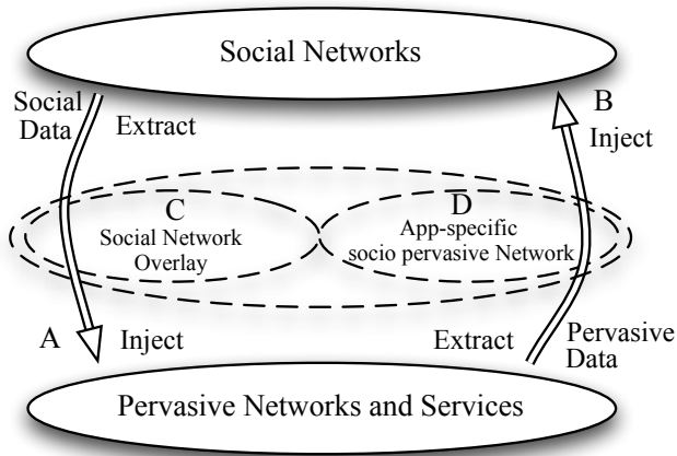
Figure 1. Approaches to integrate social sensing and pervasive services.
