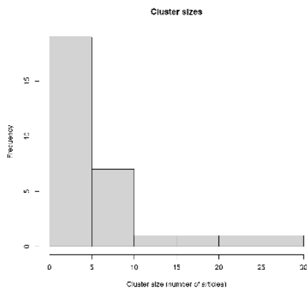
Figure 4: Cluster size distribution.
