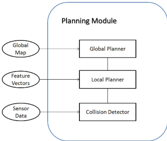
Fig. 5 Planner architecture
