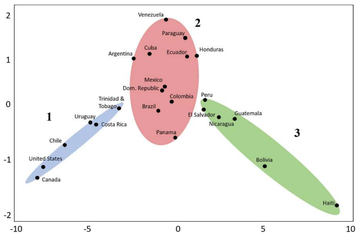
Figure A1. Results from cluster analysis of study nations based on historical values (1996–2015) of GDPP, ACSAT, and RL (R Package https://uc-r.github.io/kmeans_clustering ).
