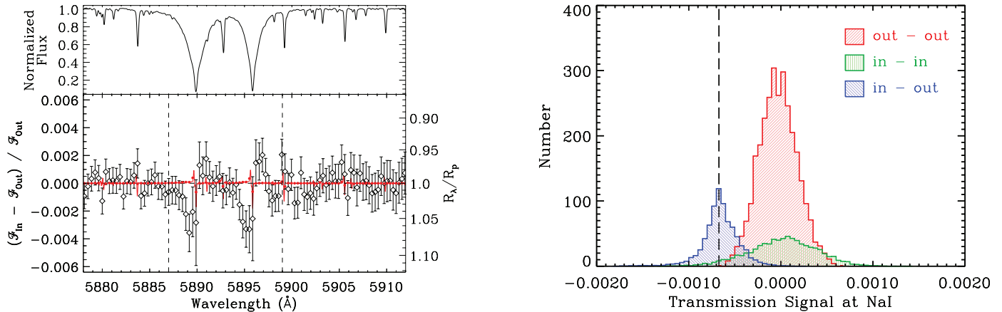
FIG. 1.— Top left: Spectrum of HD 189733 near the Na I doublet. Bottom left: The difference of the relative flux of the in-transit template ( \mathcal{F}_{in} ) and the out-of-transit template ( \mathcal{F}_{out} ). Excess absorption in the in-transit template is clearly detected in both Na I lines. Also shown is the contribution of differential limb darkening (red line and filled circles), which has been removed from the data, but the effect is minimal. The vertical dashed lines indicate the narrow bandpass used to calculate the relative transmission spectrum absorption and is identical to that used by Charbonneau et al. (2002). The right-hand axis gives the effective radius of the planet as a function of wavelength, assuming stellar and planetary properties from Pont et al. (2007). Right: Distributions of the empirical Monte Carlo analysis, which demonstrate the stability of the observations and the contribution of systematic errors. The full data set transmission spectrum absorption measurement is indicated by the vertical dashed line. Given the random and systematic errors measured by the standard deviation of the “out-out” distribution, this exoplanetary absorption detection is >3 \sigma .
