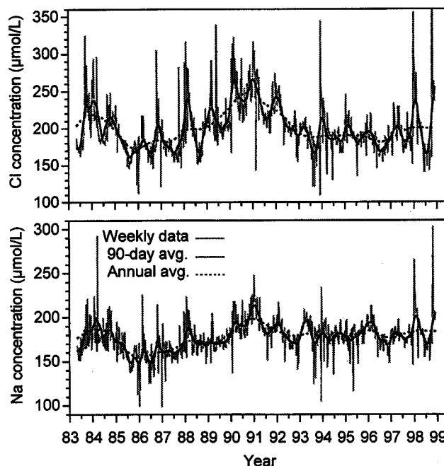
Fig. 3. Concentrations of chloride (top panel) and sodium (bottom panel) in lower Hafren streamflow. Weekly measurements are shown in grey and 90-day averages are shown by black solid and dotted lines, respectively. Sodium concentrations are less variable than chloride, on all timescales. The chloride concentration scale has been compressed by the sea-salt sodium/chloride ratio (0.86) to make the two scales comparable.
