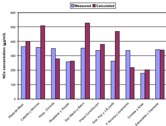
Figure 5 – Comparison between monitoring campaign and model results for \text{NO}_x maximum hourly concentration in 10 stations (fall 2000).
