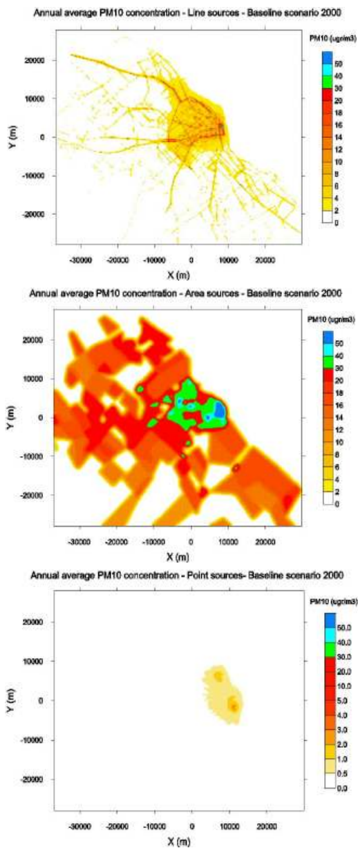
Figure 10 – PM 10 contribution by source: Line (upper), Area (middle) and Point (lower). Blue zones indicate annual average PM 10 levels exceeding 50 µg/m 3 .
