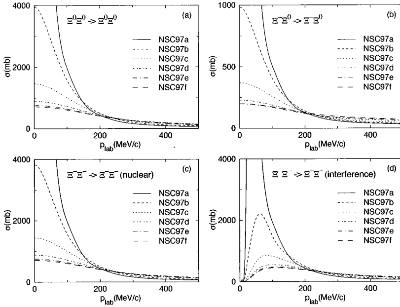
FIG. 6. Prediction of the total cross section in mb for (a) \Xi^0\Xi^0 , (b) \Xi^-\Xi^0 , (c) purely nuclear \Xi^-\Xi^- , and (d) \Xi^-\Xi^- scattering including the Coulomb-nuclear interference modification.
