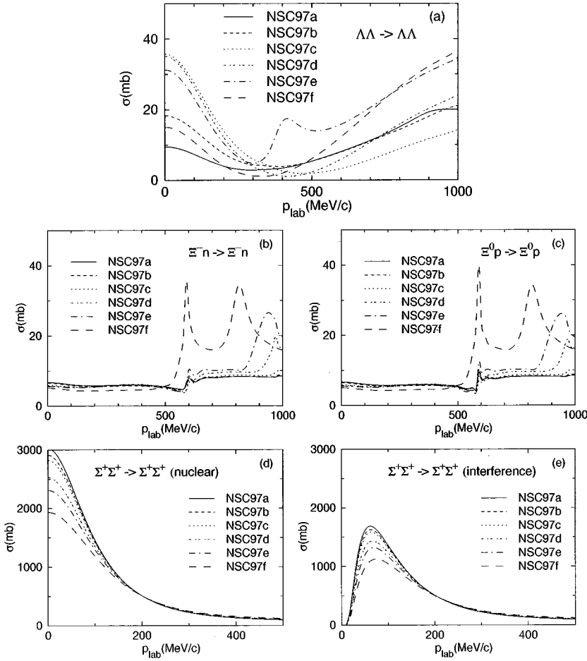
FIG. 4. Prediction of the total cross section in mb for (a) \Lambda\Lambda , (b) \Xi^-n , (c) \Xi^0p , (d) purely nuclear \Sigma^+\Sigma^+ , and (e) \Sigma^+\Sigma^+ scattering including the Coulomb-nuclear interference modification. The nuclear and Coulomb-nuclear interference results for \Sigma^-\Sigma^- scattering are practically identical to the corresponding \Sigma^+\Sigma^+ cases and, hence, are not shown explicitly.
