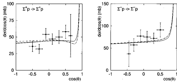
FIG. 3. Predictions for differential cross sections at p_{\Sigma^{+}} = 170 MeV/c and p_{\Sigma^{-}} = 160 MeV/c for models NSC97a (solid line), NSC97c (dotted line), and NSC97f (dash-dotted line). Experimental data from Ref. [52].
