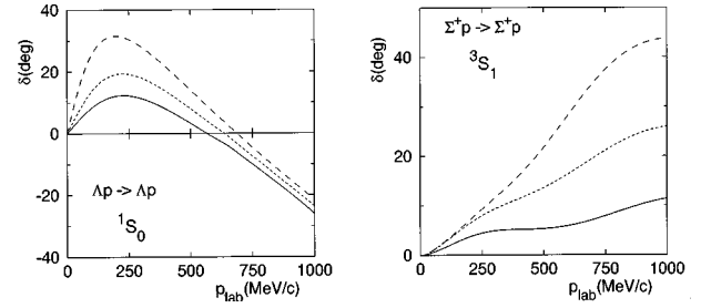
FIG. 4. \Lambda p ^1S_0 and \Sigma^{+}p ^3S_1 phase shifts for models NSC97a (solid line), NSC97c (dotted line), and NSC97f (dash-dotted line).
