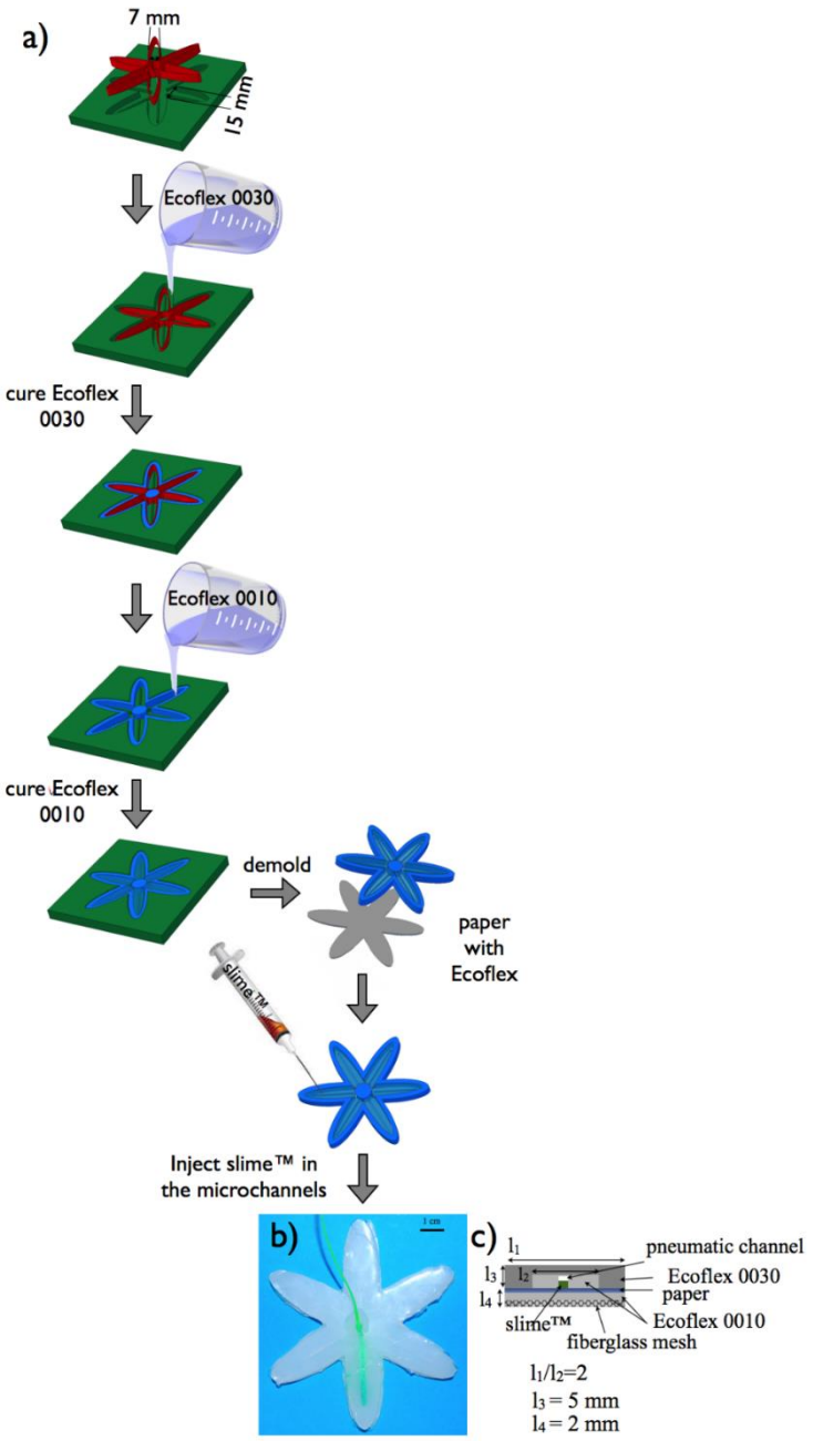
Figure S4. a) Schematic diagram of soft gripper assembly. b) Top face view of a gripper with a channel filled with slime™. c) Profile scheme of a gripper arm.
