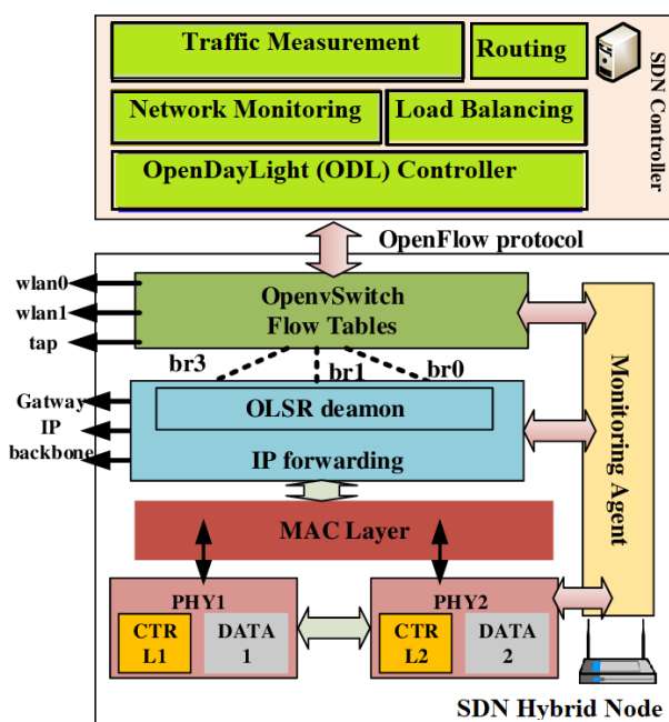
FIGURE 6. The SDN Hybrid Node Architecture
