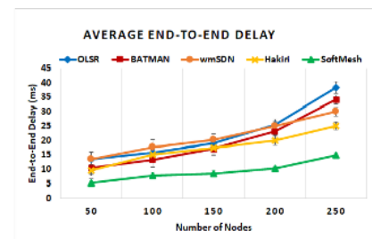
b) Scenario 02 (25% SDN hybrid nodes + 75% Legacy nodes)
