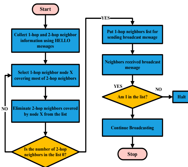
FIGURE 10. Working of Legacy Node
