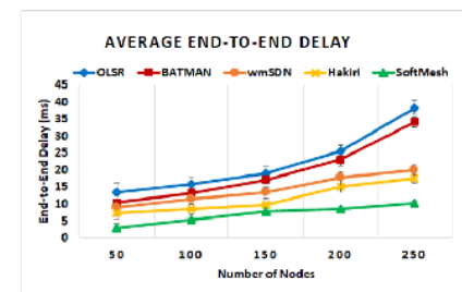
c) Scenario 03 (50% SDN hybrid nodes + 50% Legacy nodes)
