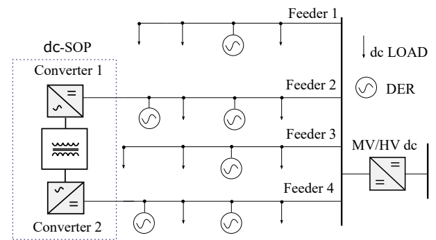
FIGURE 7. Basic topology of dc-SOP.
