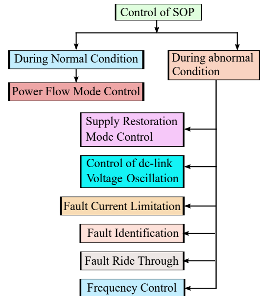
FIGURE 10. Summary of Control of SOP in DNs.
