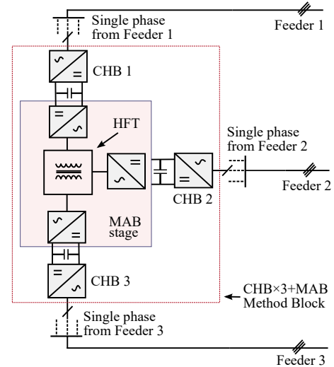
FIGURE 9. Simplified block diagram of CHB×3+MAB method for a single phase line.
