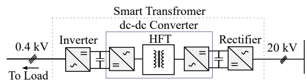
FIGURE 3. Basic Configuration of smart transformer in DNs.
