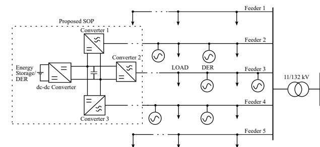
FIGURE 6. Basic topology of SOP+ES.
