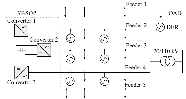
FIGURE 5. Basic topology of 3T-SOP in DNs.
