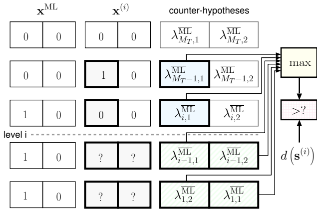
Fig. 2. Example of the STS pruning criterion ( M_T = 5 and two bits per symbol): The partial binary label \mathbf{x}^{(i)} determines which counter-hypotheses may be affected during the search of the subtree emanating from the current node.
