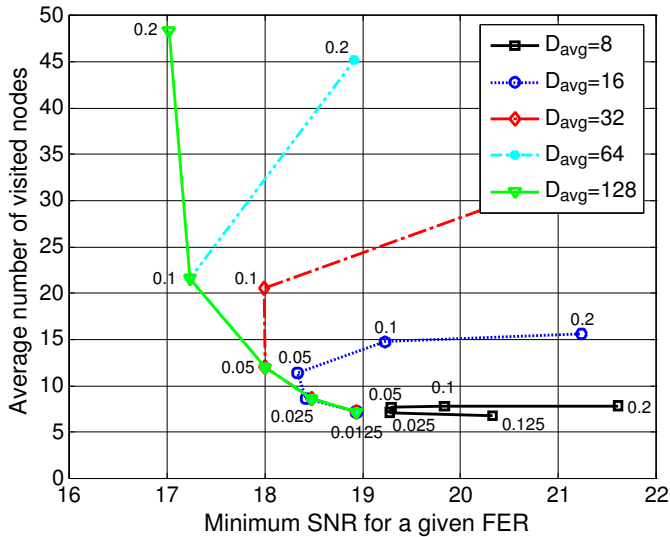
Fig. 5. Impact of run-time constraints with MF scheduling on STS SED with MMSE-SQRD preprocessing at a FER of 0.01. The performance can be optimized by choosing an appropriate LLR clipping level (shown next to the curves) for a given average run-time constraint D_{avg} .
