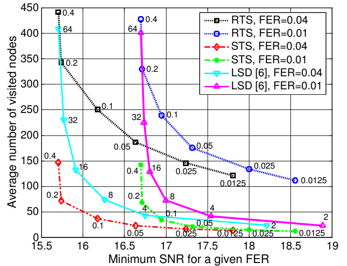
Fig. 3. Comparison of repeated tree search (RTS), single tree search (STS) and the list sphere decoder (LSD) as proposed in [6]. The numbers next to the curves correspond to L_{\text{max}} for RTS and STS and to the list size in the case of the LSD.
