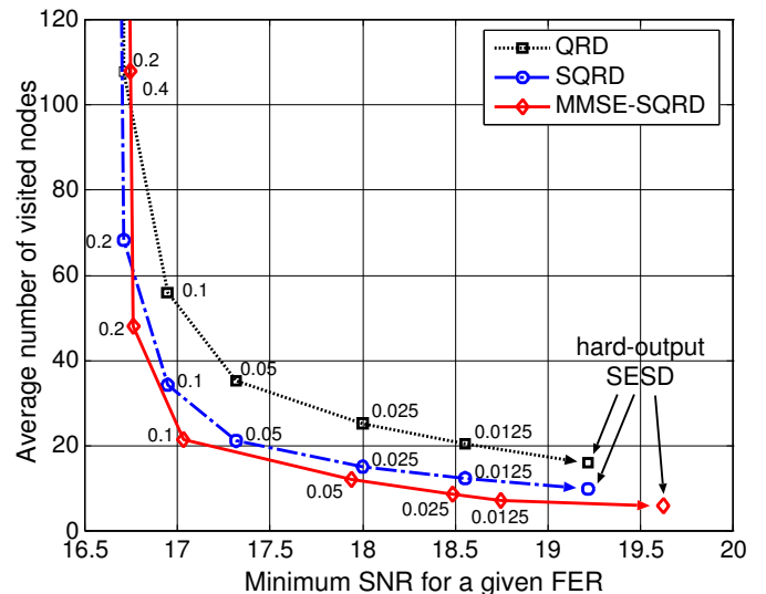
Fig. 4. Comparison of unordered QRD, SQRD and MMSE-SQRD preprocessing applied to STS at a target FER of 0.01. The numbers next to the curves correspond to L_{\text{max}} . For L_{\text{max}} \rightarrow 0 , the performance approaches that of hard-output SESD.
