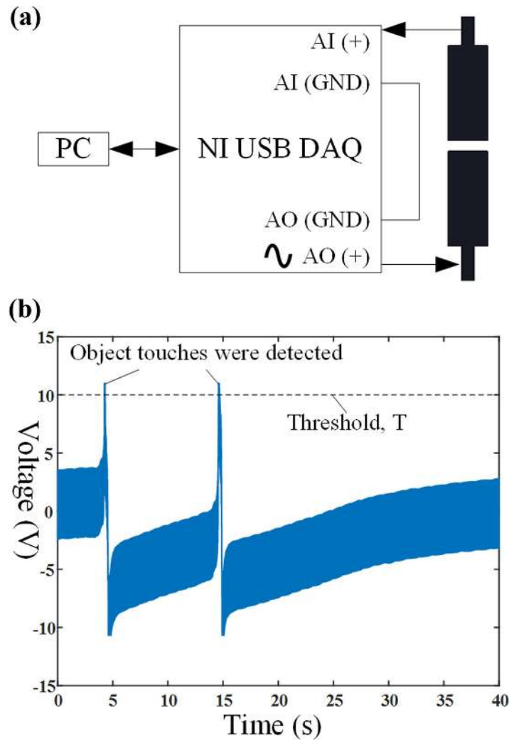
Figure 10. The soft touch sensor: (a) schematic diagram and (b) sensor reading when there is no object and there is an object touching the sensor.
