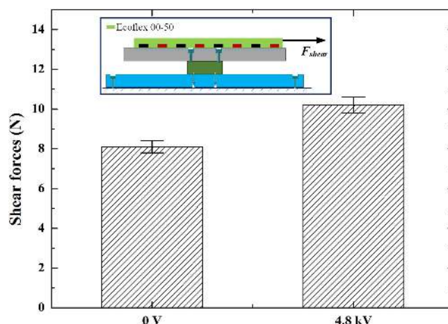
Figure 5. Shear adhesive forces of the soft electroadhesive gripper under 0 V and 4.8 kV.
