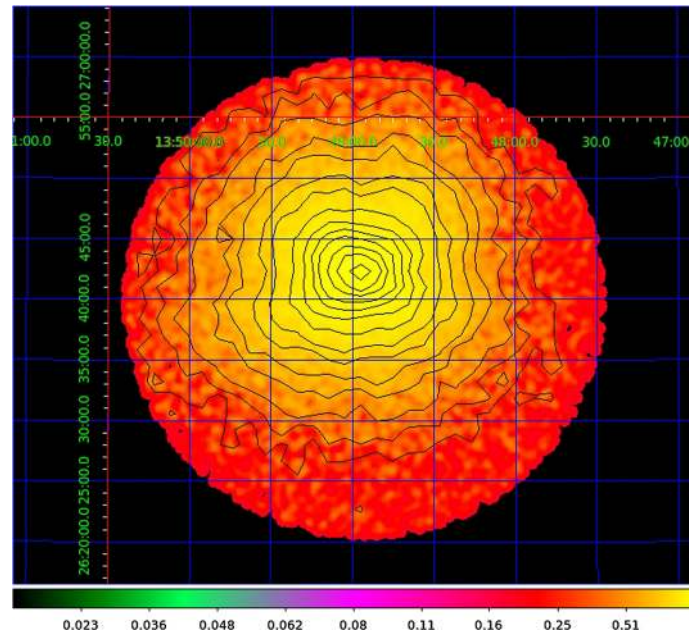
Figure 10. SXT image of Abell 1795 cluster of galaxies after a slight smoothing using a Gaussian function, \sigma = 40 arcsec.
