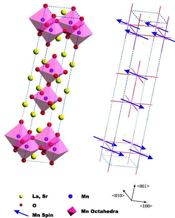
FIG. 1 (color online). The magnetic and crystallographic structure of the Ruddlesden-Popper bilayer manganite \text{La}_{2-2x}\text{Sr}_{1+2x}\text{Mn}_2\text{O}_7 .
