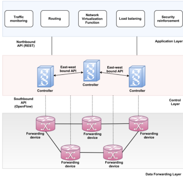
Fig. 2. SDN Architecture
