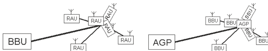
Figure 2. C-RAN (left) vs. D-RAN architecture (right).
