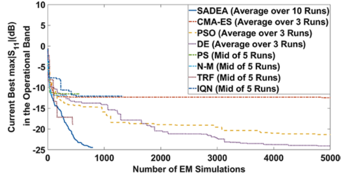
Fig. 6. Convergence graphs of all methods (Example 2).
