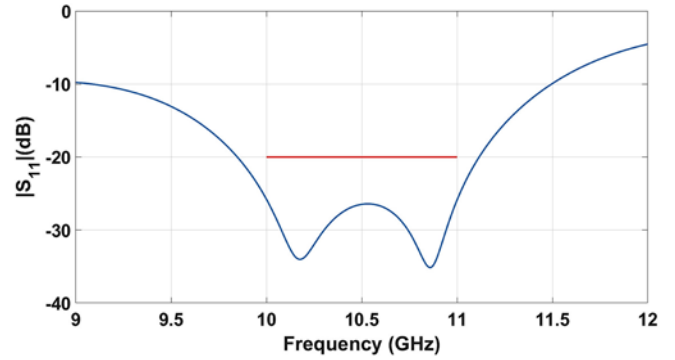
(a) S_{11} versus frequency.
