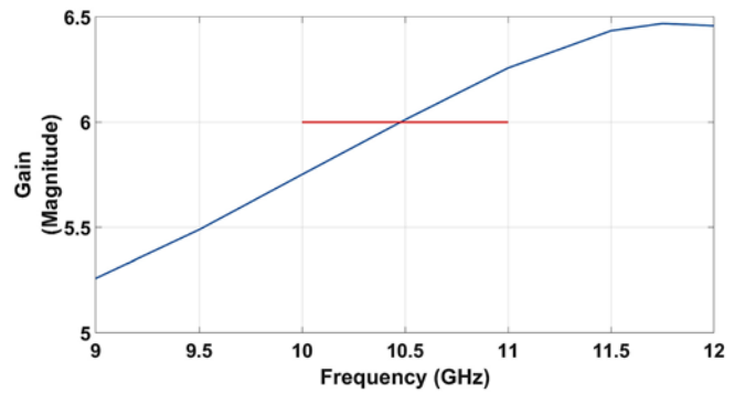
(b) Gain versus frequency.
