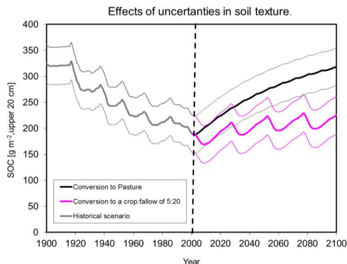
Fig. 6. Effects of data uncertainty during modelling of the potential impact on soil organic carbon from land use management. Result from a Monte Carlo simulation ( n=500 ) assuming a data uncertainty in the soil clay content (mean = 5% and \sigma=2.5\% ). Thick lines describe simulation without data uncertainty and the thin lines describe the output distribution (95%) from the Monte Carlo simulation (calculated as the output standard deviation from the Monte Carlo simulation ( 18 ) \times 1.96 = 36 ). The black line describes effects on SOC assuming grazing only and the blue line describe effects on SOC assuming a traditional Millet cropping system with 5 year of cultivation and then 20 years of fallow.
