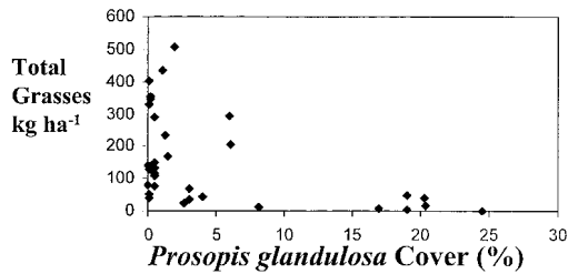
Fig. 3. Relationship between total perennial grass production and mesquite canopy cover on the Chihuahuan Desert Rangeland Research Center in south central New Mexico using data pooled across years (1995, 1996, 1997).
