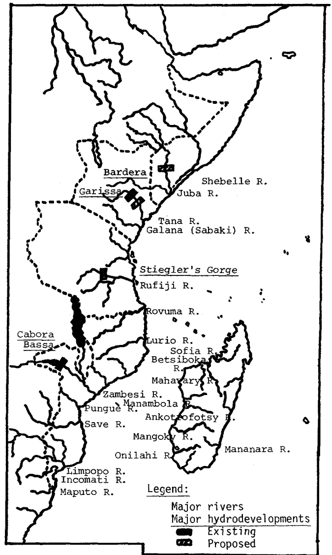
FIG. 2. MAJOR RIVERS AND HYDRODEVELOPMENT PROJECTS
