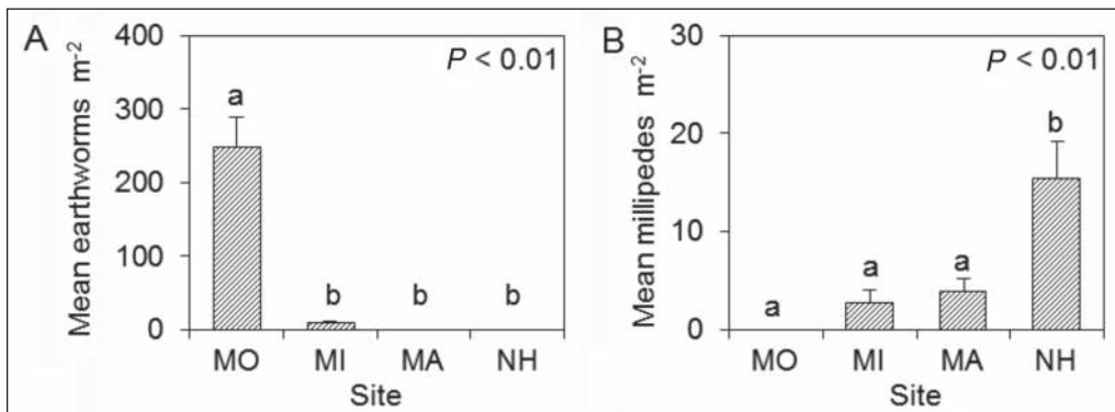
Figure 2. Mean (A) earthworm and (B) millipede abundances for soil and litter combined at 4 sites in the eastern US. Bars with different letters above are significantly different at \alpha = 0.05 ; error bars represent the standard error of the mean. Note differences in y-axis scales. Site abbreviations are as in Figure 1.
