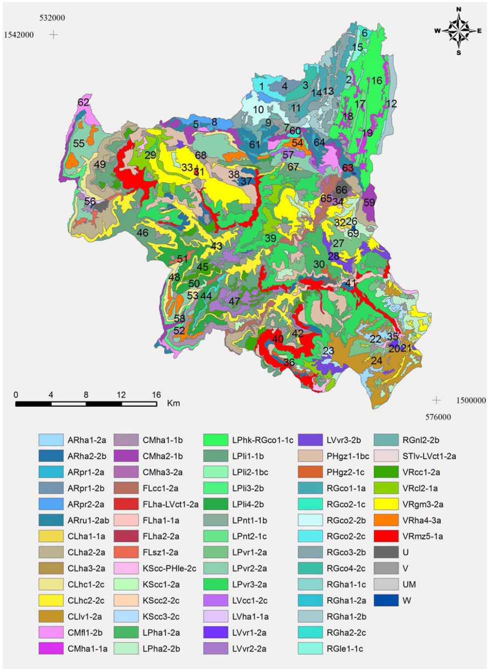
Figure 2 - Soil map according to FAO-UNESCO (1988) classification system
