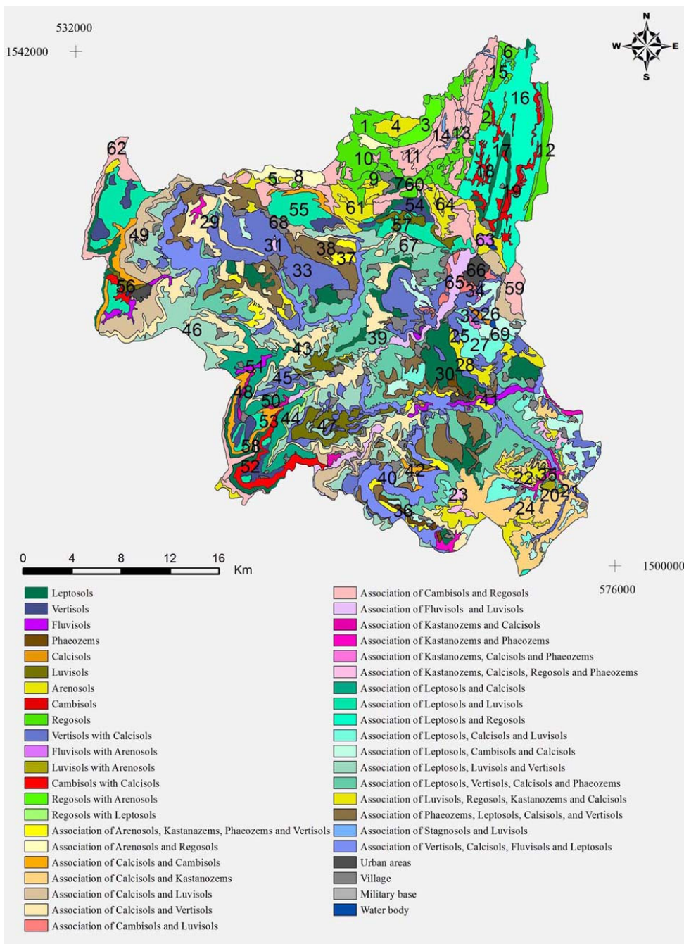
Figure 3 - Soil map according to WRB 2006 classification system
