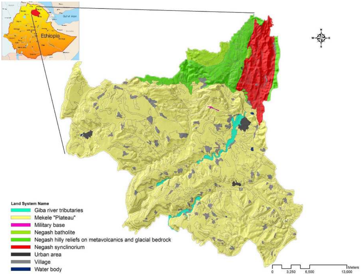
Figure 1 - Land Systems of the study area
