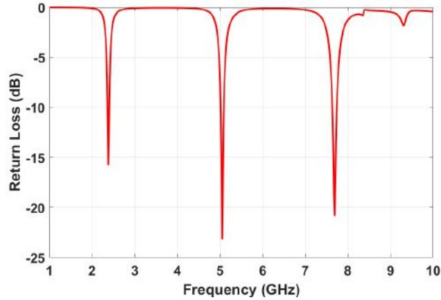
Figure 15. SIW-cavity MPA's return loss before etching channels
