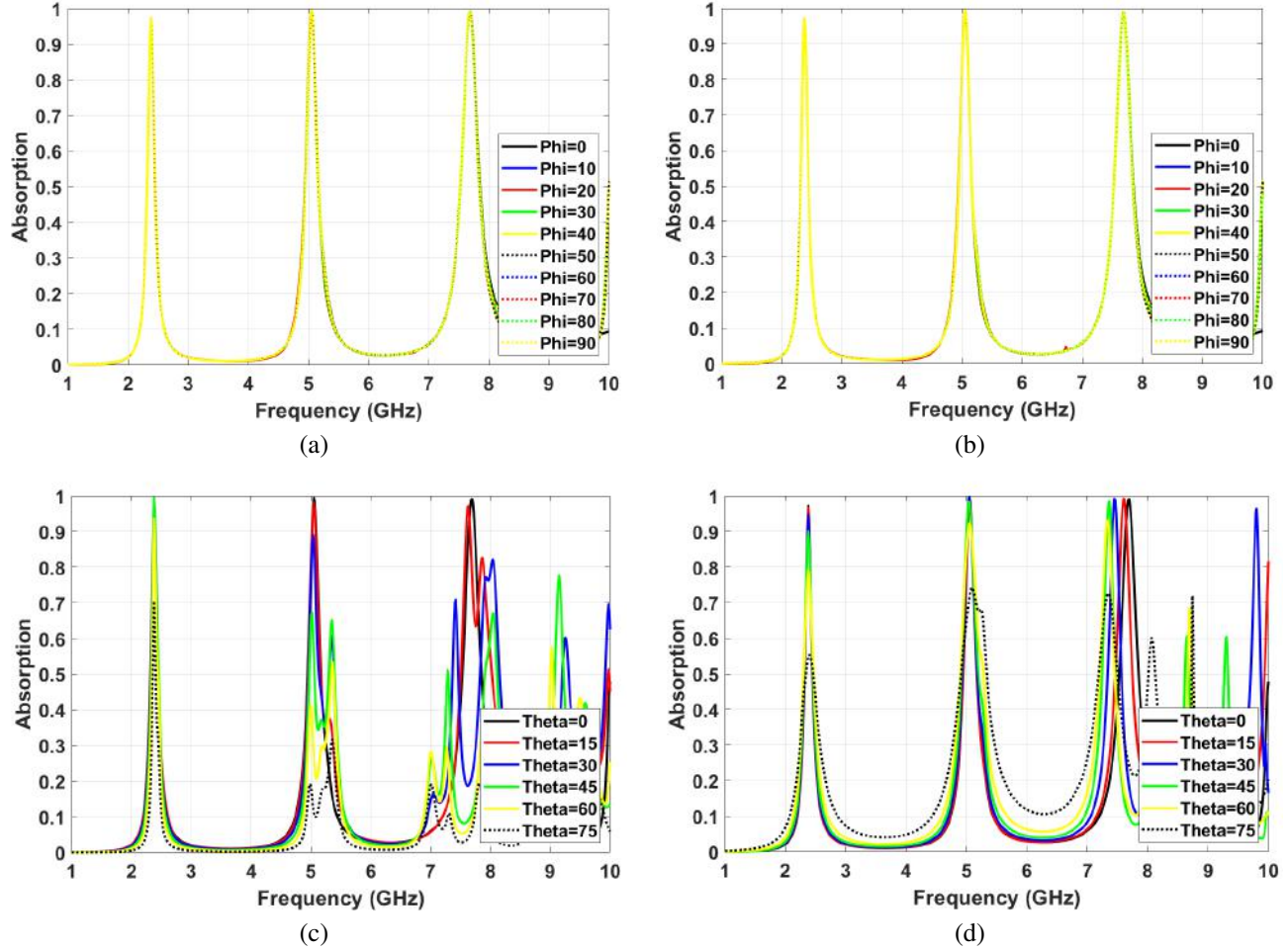
Figure 8. Angle insensitivity (a) Different polarization angles for TE waves, (b) Different polarization angles for TM waves, (c) Different incident angles for TE waves, (d) Different incident angles for TM waves
