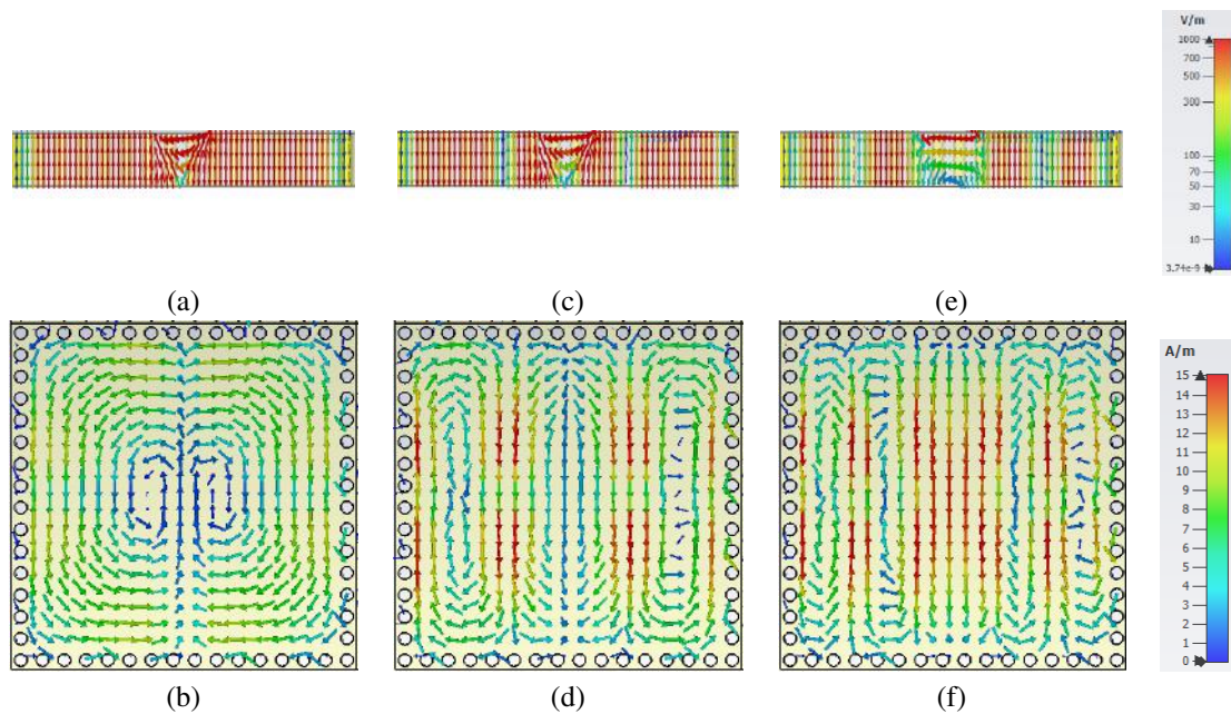
Figure 5. Electromagnetic fields facing TM polarized incident waves (a) E-field distribution at f = 2.4 \text{ GHz} ( TE_{201} ), (b) H-field distribution at f = 2.4 \text{ GHz} ( TE_{201} ), (c) E-field distribution at f = 5 \text{ GHz} (Hybrid mode of TE_{201} and TE_{401} ), (d) H-field distribution at f = 5 \text{ GHz} (Hybrid mode of TE_{201} and TE_{401} ) (e) E-field distribution at f = 7.7 \text{ GHz} ( TE_{401} ), (f) H-field distribution at f = 7.7 \text{ GHz} ( TE_{104} )
