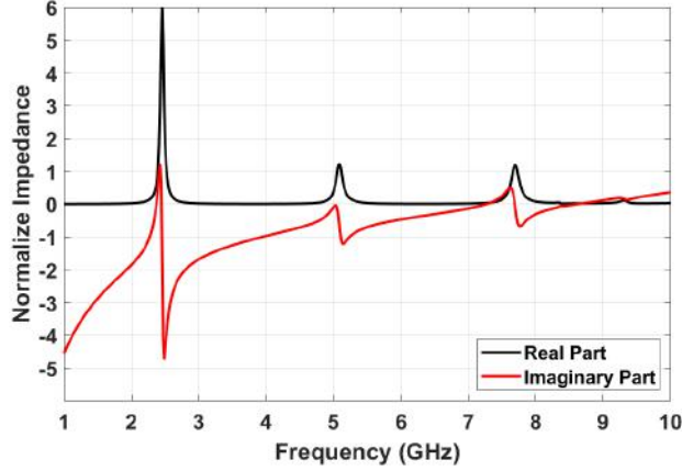
Figure 6. Input impedance of SIW cavity resonator
