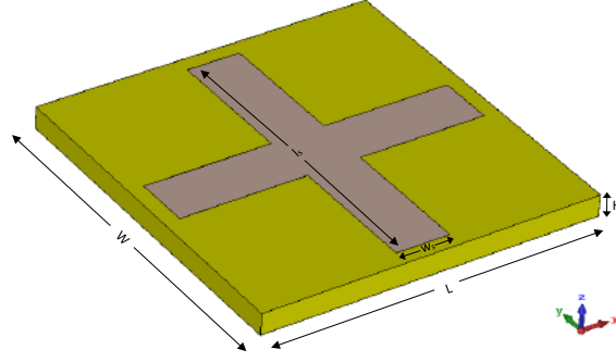
Figure 1. Cavity resonator MPA unit cell
