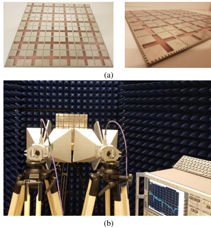
Figure 12. (a) Fabricated 6 \times 6 MPA, (b) Implemented measurement setup.
