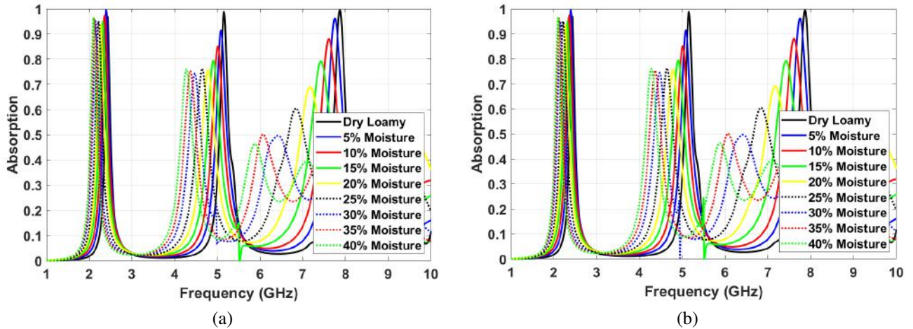
Figure 11. Sensing efficiency of the proposed MPA for different moisture levels in Loamy soil (a) facing TE polarized incident waves, (b) facing TM polarized incident waves
