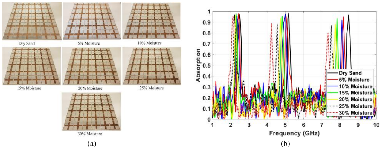
Figure 14. Measuring of sensing capability (a) Filling MPA channels by sand with different levels of moisture, (b) Changing absorption characteristics by varying the soil moisture.
