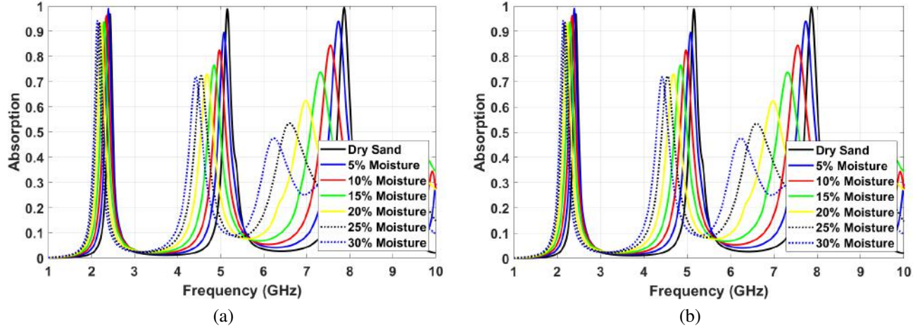
Figure 10. Sensing efficiency of the proposed MPA for different moisture levels in sand soil (a) facing TE polarized incident waves, (b) facing TM polarized incident waves
