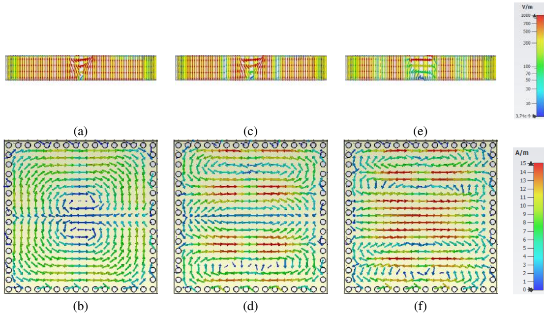
Figure 4. Electromagnetic fields facing TE polarized incident waves (a) E-field distribution at f = 2.4 \text{ GHz} ( TE_{102} ), (b) H-field distribution at f = 2.4 \text{ GHz} ( TE_{102} ), (c) E-field distribution at f = 5 \text{ GHz} (Hybrid mode of TE_{102} and TE_{104} ), (d) H-field distribution at f = 5 \text{ GHz} (Hybrid mode of TE_{102} and TE_{104} ) (e) E-field distribution at f = 7.7 \text{ GHz} ( TE_{104} ), (f) H-field distribution at f = 7.7 \text{ GHz} ( TE_{104} )
