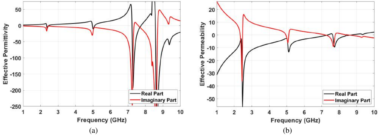
Figure 7. (a) Effective permittivity , (b) Effective permeability
