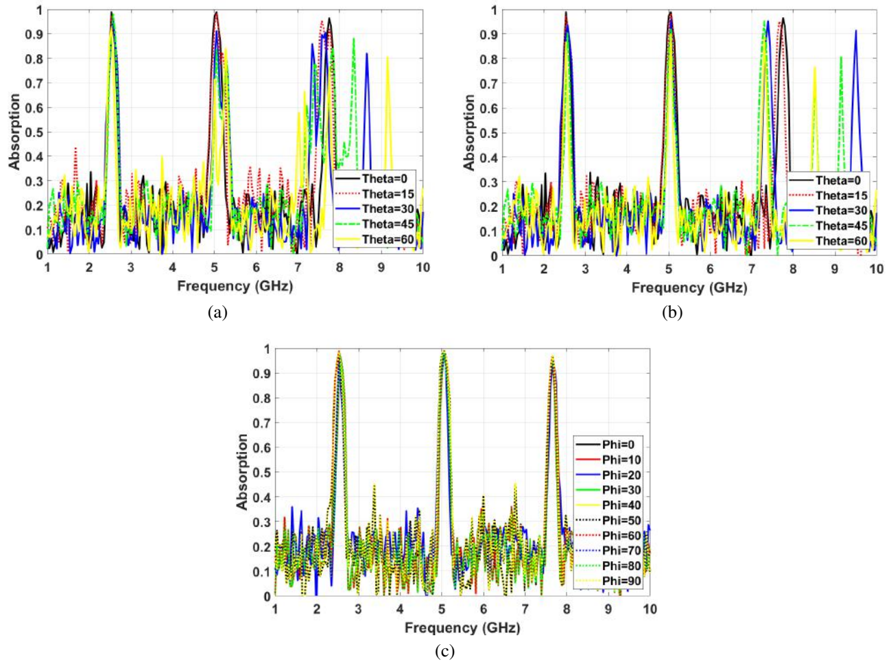
Figure 13. Angle insensitivity measurement results (a) Different incident angles for TE waves, (b) Different incident angles for TM waves, (c) Different polarization angles
