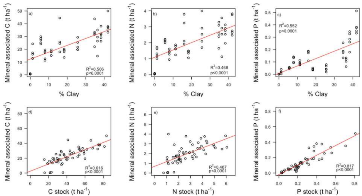
Figure 3. Mineral associated carbon (C) Nitrogen (N), phosphorus (P), and isolated by density and size fractionation and their association with, (a–c) clay (<math> < 2 \mu\text{m}</math>) content of the soil, and (d–f) total elemental stocks in the top 15 cm of the soil. Stocks were calculated by multiplying elemental concentrations by bulk density.
