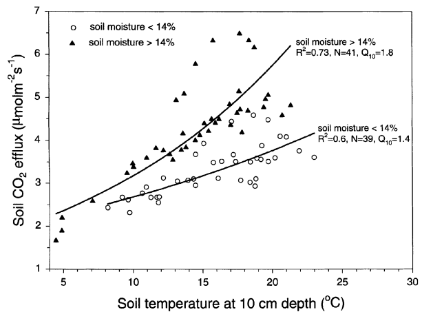
Fig. 3 The effect of soil moisture on the relationship between soil CO 2 efflux and soil temperature. High Q 10 value corresponds to high soil moisture. Each datum represents the average over 18 measurement locations.
