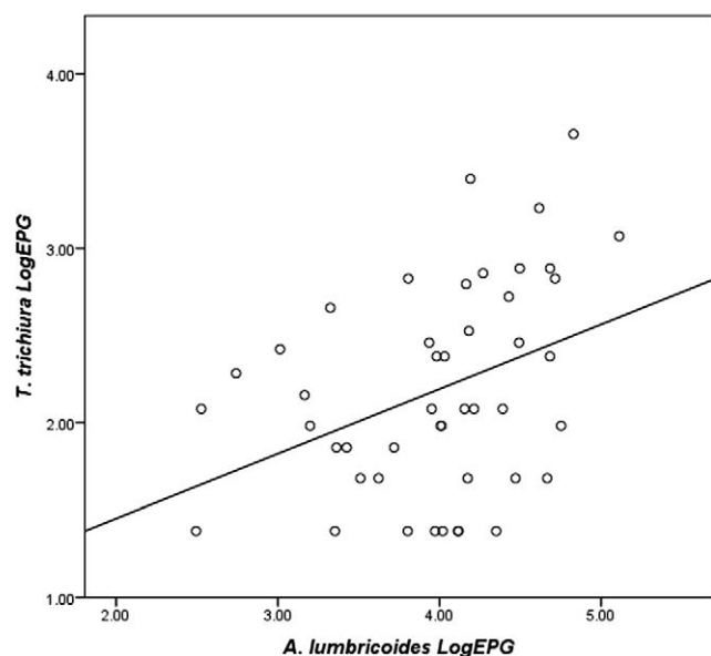
FIGURE 2. Correlation between Trichuris trichiura and Ascaris lumbricoides infection intensity. Values represent logEPGs for T. trichiura and A. lumbricoides among infected individuals ( R^2 = 0.143 ).
