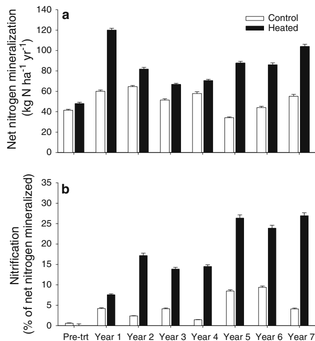
Fig. 1 a Net N mineralization in the control (open bars) and heated (filled bars) areas. Bars represent mean net N mineralization rates of subplots ( n = 10 ) in kg N ha -1 year -1 + 1SE. b Net nitrification as a percent of total net N mineralized. Bars represent mean net N mineralization rates in percent of subplots ( n = 10 ) + 1SE
