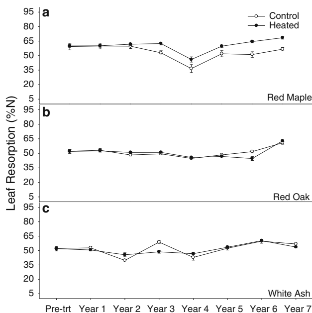
Fig. 4 Average percent N resorption for a red maple b red oak and c white ash in the control (open circles) and heated (filled circles) areas. Lines represent %N values retained in the trees during senescence by species \pm 1\text{SE} . A pre-treatment correction factor was applied to the resorption values
