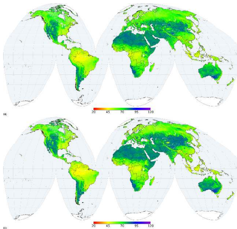
Figure 10. Prediction distribution for \text{pH}_{\text{water}} (10 pH) in the 60 to 100 cm depth interval, (a) for 5% quantile and (b) for 95% quantile.
