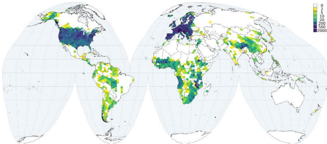
Figure 4. Number of observations per grid cell ( 70\,000\text{ km}^2 ) for coarse fragments.
