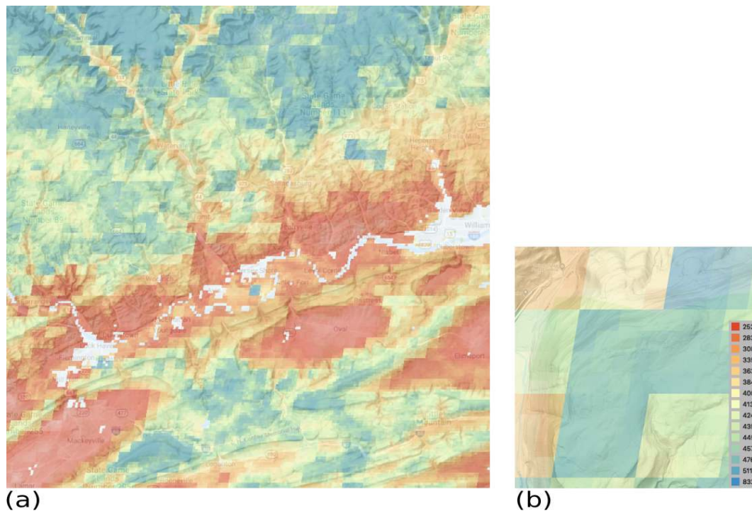
Figure 6. Predicted sand concentration, %, 0–5 cm, ground overlay in © Google Earth. (a) Overview; centre \approx -77^{\circ}14' E, 41^{\circ}14' N , near Jersey Shore, PA. (b) Detail; centre \approx -76^{\circ}56' E, 41^{\circ}33' N .
