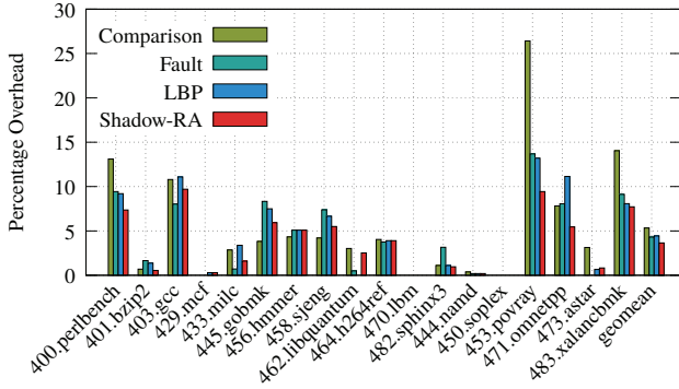
Fig. 9: Epilogue Micro-Optimizations
