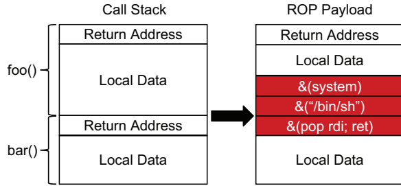
Fig. 1: ROP Illustration
