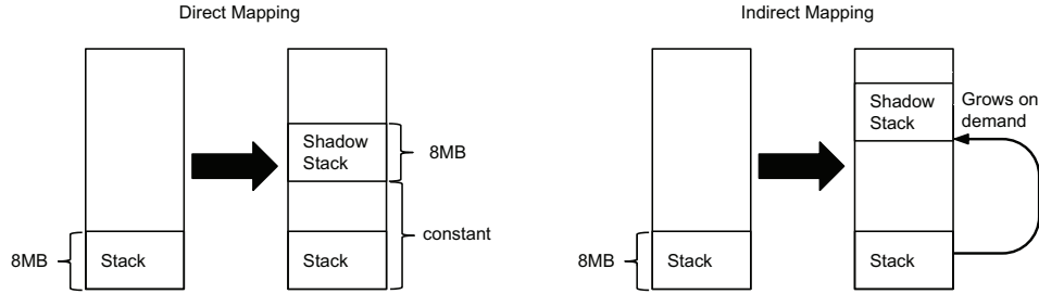
Fig. 2: Shadow Stack Designs – Mapping Options
