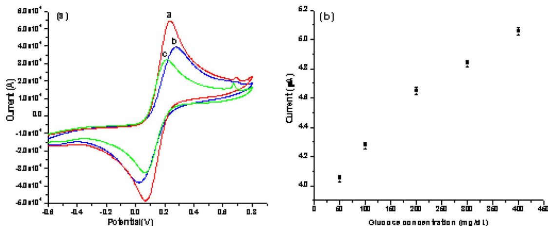
FIG. 3. (Color online) Cyclic voltammograms of (a) curve a; bare Au electrode, curve b; CeO 2 /Au electrode, curve c; GOx/CeO 2 /Au bioelectrode. (b) Amperometric response of GOx/CeO 2 /Au bioelectrode as a function of glucose concentration.
