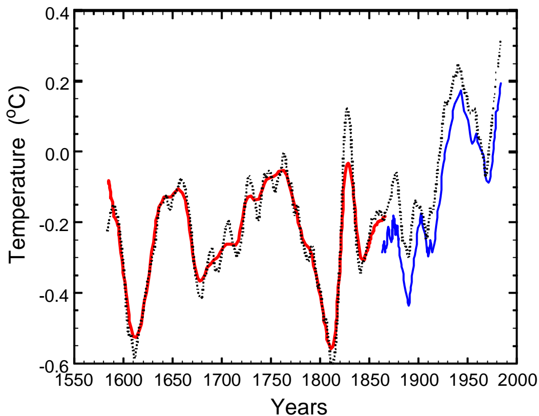
Figure 7: 11-year running average of the Groveman / Landsberg / Borzenkova temperature series 1579-1975 (dotted line) presented in Groveman and Landsberg (1979). Simplified version 1585-1866 of the 11-year running average of the Groveman / Landsberg / Borzenkova temperature series (red solid line) as employed by Lassen and Friis-Christensen (1995). The precise definition of curve is unclear since it does not correspond to the authors' description. 11-year running average of temperature series 1862-1982 (blue solid line) from Jones et al. (1986), Jones (1988) and Jones et al. (1998). The Jones curve describes a temperature variation, which is very similar to the corresponding part of the Groveman / Landsberg / Borzenkova curve apart from a downward displacement by 0.1°C because the Jones series employs a different temperature scale. In order to make comparisons easier the Groveman / Landsberg / Borzenkova curve has been extended so that it ends in the same year as the Jones curve. This has been achieved by adding zero-point adjusted Jones data for 1975-1982.
