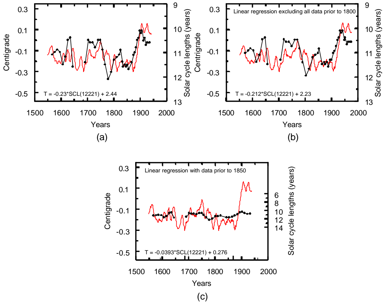
Figure 8: (a) Solar cycle lengths (black line with solid circles) fitted to Northern Hemisphere land temperatures as presented by Lassen and Friis-Christensen (2000) (red solid line). Here the solar data density after year 1850 (i.e. over the time period where both curves exhibit the above mentioned ‘S-shape’) has been doubled by adding maximum-maximum cycle lengths to the minimum-minimum cycle lengths previously employed. Thereby a good agreement has been achieved over just the period where man-made greenhouse gases may have caused a global warming trend which is superimposed over the natural temperature fluctuations, whereas the earlier data which are not affected by human influences only show a poor agreement. Hence, the displayed partial agreement may primarily be the consequence of: (1) a certain, spurious similarity in shape of the solar curve and the development of human industrial activity over time and (2) the employment of a (linear regression) scaling factor which does not take into account data outside this specific period. This interpretation is supported by the fact that the agreement of the solar curve and temperature curve is poor before 1870. The problematic utilization of this ‘S-shape similarity’ is also illustrated on Fig. 5 above where the flat S-shape of the solar curve can be scaled up so as to agree with the steep S-shape of the temperature curve inside the inserted frame. But this special choice of scaling parameter would lead to an unacceptable mismatch of the two curves outside the inserted frame. (b) The result of a test calculation, one of a series of test calculations performed in order to determine the numerical weight factors which Lassen and Friis-Christensen (2000) have applied to the older solar data. The numerical values of these factors are not given by the authors. Fig. 8.b is obtained by tentatively putting to zero all weight factors of solar data prior to year 1800. It is seen to be practically identical with Fig. 8.a . Normally data with a weight factor zero would be omitted, since data, which are deemed too unreliable to be taken into account in a linear regression will not be presented together with valid data, or at least not without warning the reader. The applied reasoning may be described as follows: First the solar and temperature curve are forced to agree over the period 1870-1960 (where the temperature curve may be strongly influenced by man-made global warming). This is done at the expense of the earlier data. And then the result is presented in a way, which suggests that the temperature rise is caused by solar and not by human activity. (c) Here the same data as in Fig. 8.a and Fig. 8.b are fitted employing linear regression, leaving out, however, the artificial doubling of the mathematical weight obtained by adding maximum-maximum cycle lengths, but retaining the early solar data and assigning equal weights to all data. However, in order to reduce ‘contamination’ from possible anthropogenic influences, only data prior to year 1850 have been used in the linear regression.
