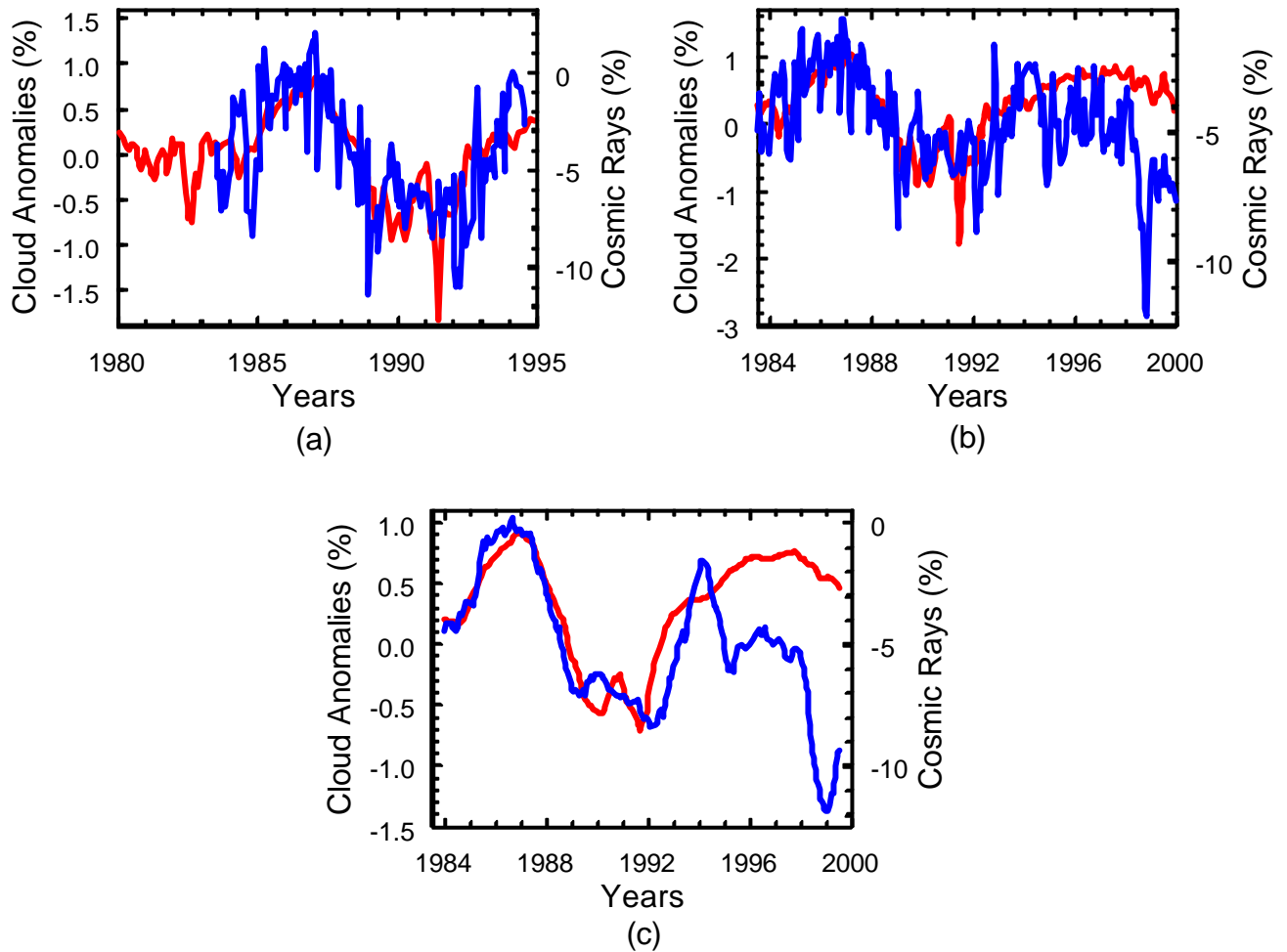
Figure 2: (a) Low cloud cover (blue solid line) and galactic cosmic ray intensity as observed at the Peruvian station Huancayo (red solid line) according to Marsh and Svensmark (2000) . (b) Low cloud cover (blue solid line) and galactic cosmic ray intensity as observed at Huancayo (red solid line) according to Kristjánsson (2002) . (c) Same as (b) but smoothed in order to display the trends more clearly.
