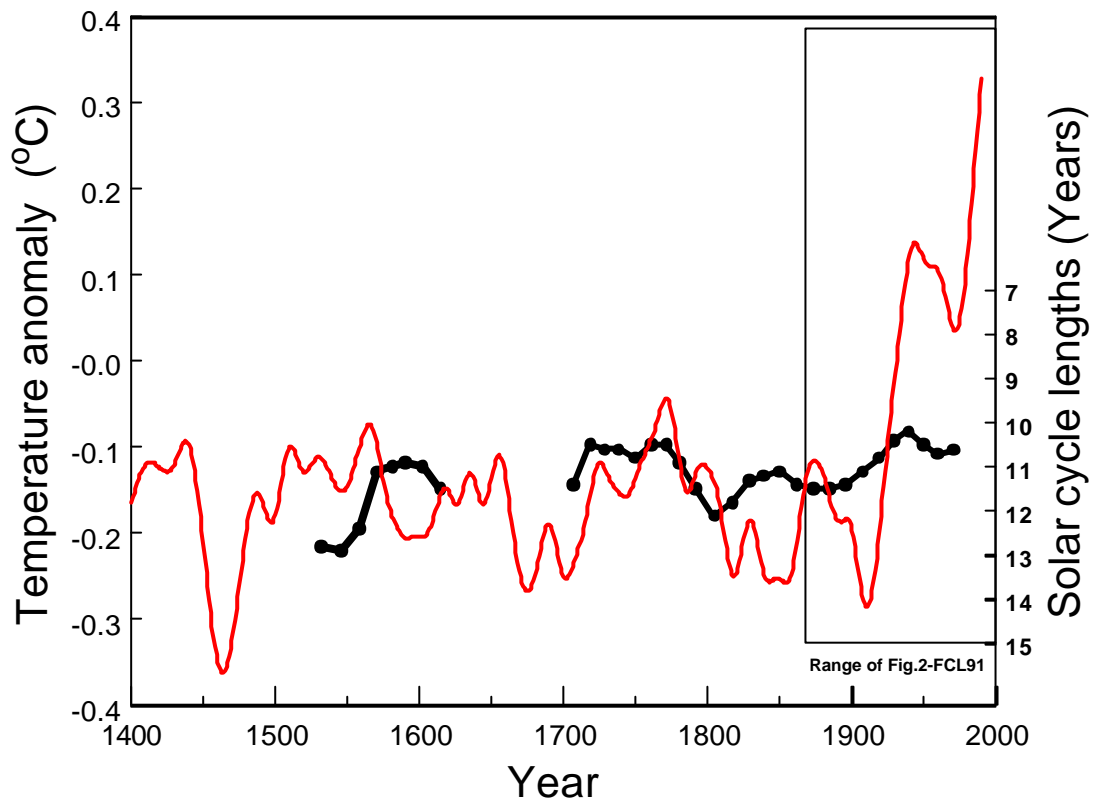
Figure 5: 1,2,2,2,1-filtered minimum-minimum solar cycle lengths (black curve with solid circles) and Northern Hemisphere land temperatures (red solid line). These are essentially the same physical parameters as on Fig. 3.a , but here they are shown over a longer time period. Notice that the method of linear regression in general gives a far less convincing agreement of the solar and terrestrial data when applied to a longer time period where each curve includes a larger number of specific details. The inserted frame indicates the range of Fig. 3.a above. It should also be noticed that a scaling that yields a better agreement of the ‘S-shapes’ of the two curves within the range of the frame (a scaling as applied on Fig. 3.a ) will make the agreement outside the range worse. This would, e.g., lead to an increased mismatch between the solar ‘top’ and the temperature ‘valley’ around 1600.
