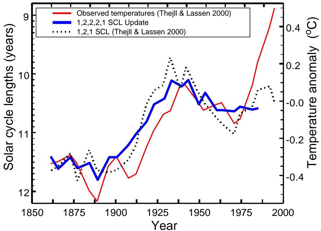
Figure 4: Observed temperatures (red thin solid line) and 1,2,1-filtered solar cycle lengths (black dotted line) as shown on Fig. 3 in Thejll and Lassen (2000) . 1,2,2,2,1-filtered solar cycle lengths as shown on Fig. 2 in Friis-Christensen and Lassen (1991) with four updated points (blue heavy solid line).
