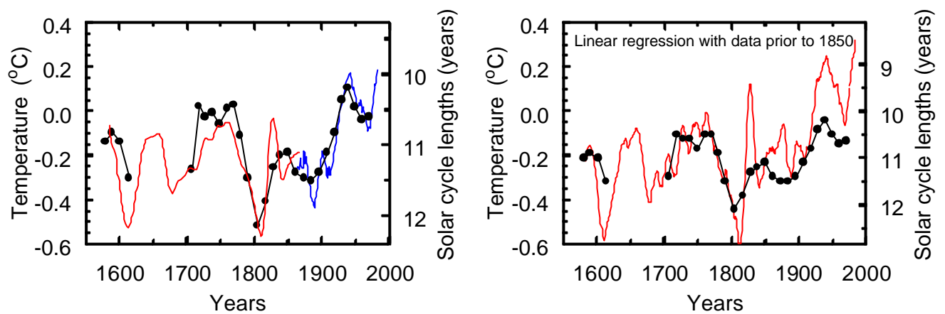
Figure 6: (a) 1,2,2,2,1-filtered minimum-minimum solar cycle lengths (black line with solid circles) and two different series of Northern Hemisphere temperatures: Grovemann / Landsberg (red solid line) and Jones (blue solid line). The seemingly good agreement of the two temperature curves with the solar curve has been obtained in the following way: (1) The two series are plotted in different scales , whereby the right hand curve is lowered by 0.1°C. This makes about one third of the global warming over the range of the curve disappear. (2) The entire solar curve has been lifted so as to achieve a good fit of the curve over the last 150 years, at the expense of the agreement of the older data. As a consequence the solar cycle lengths on the left hand side are positioned too high. (b) Here the solar data are the same as on Fig. 6.a, but the two different temperature series employing different temperature scales are here replaced by a single series (the Groveman / Landsberg / Borzenkova series) with all temperatures measured in the same scale (red solid line). In order to make comparisons easier the Groveman / Landsberg / Borzenkova curve has been extended so that it ends in the same year as the Jones curve. This has been achieved by adding zero-point adjusted Jones data for 1975-1982. The curve fitting is here done by simple linear regression without manual adjustment, but only employing data before 1850 in order to avoid ‘contamination’ from man-made greenhouse gases.
