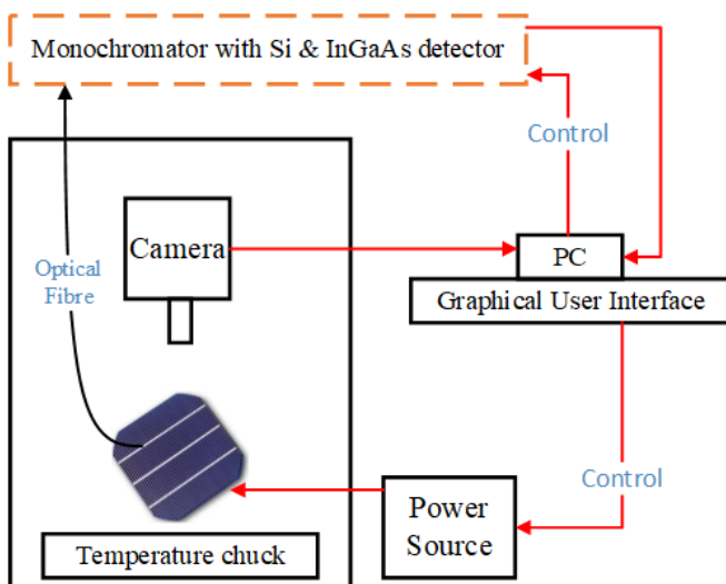
Fig. 1. Typical EL imaging system
